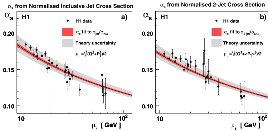
Fig. 7 The \alpha_s(\mu_r = \sqrt{(Q^2 + P_T^2)}/2) values determined using the normalised inclusive jet cross sections (a) and the 2-jet cross sections (b), each measured in 24 bins of Q^2 and P_{T,obs} . The error bars denote the total experimental uncertainty of each data point. In each plot, the solid line shows the two loop solution of the renormalisation group equation,
