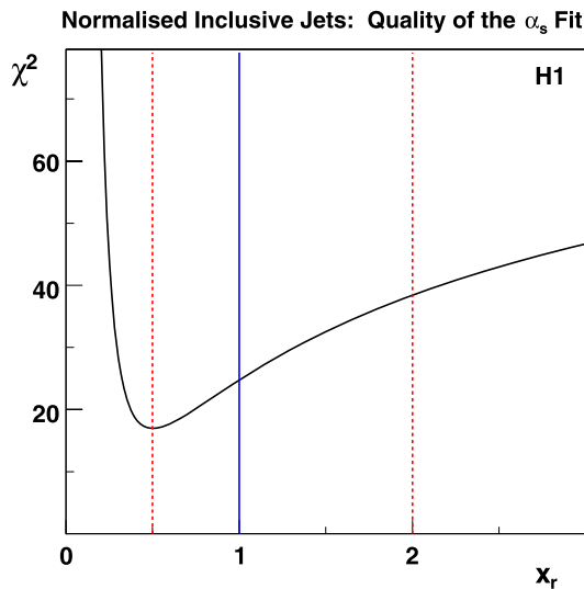
Fig. 11 The minimal \chi^2 of the fit of the NLO prediction with \mu_r = x_r \cdot \sqrt{(Q^2 + P_T^2)}/2 to the normalised inclusive jet cross section as function of x_r for 23 degrees of freedom. Vertical dashed lines represent the range where the renormalisation scale is varied in order to estimate the impact of missing orders beyond NLO, while the full line indicates the nominal choice of the scale with x_r = 1
