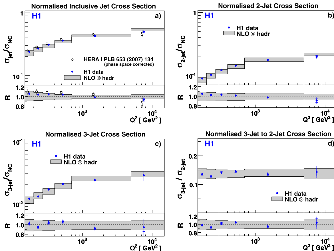
Fig. 3 The normalised inclusive jet (a), 2-jet (b) and 3-jet (c) cross sections in NC DIS measured as a function of Q^2 . The ratio of 3-jet to 2-jet cross sections is shown in (d). The measurements refer to the phase-space given in Table 1. The points are shown at the average value of Q^2 within each bin. For the inclusive jets the present data (solid dots) are compared to HERA-I published data [3], here shown corrected to the same phase space as the present measurement and shifted in Q^2 for clarity (open dots). The inner error bars represent the statistic
