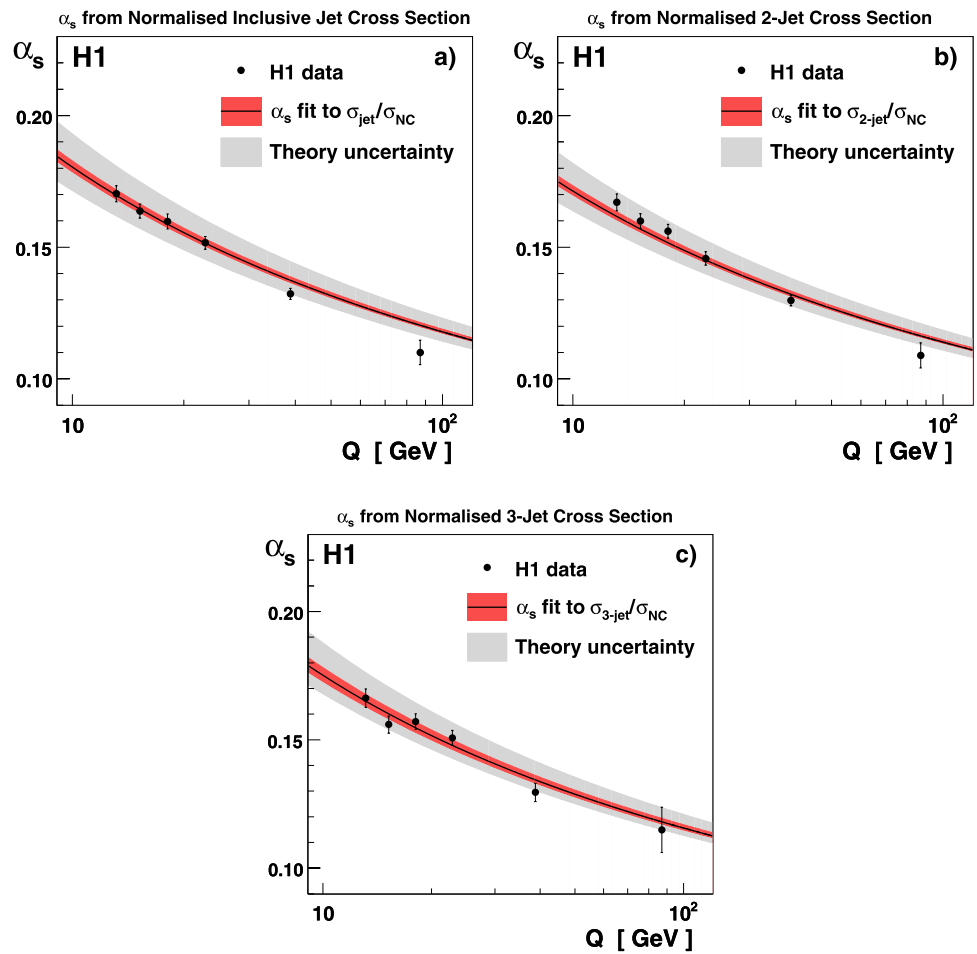
Fig. 10 The \alpha_s(Q) values extracted by fitting the P_T dependence of the normalised inclusive jet cross section in different regions of Q^2 (a); \alpha_s(Q) values extracted by fitting the \langle P_T \rangle dependence of the normalised 2-jet cross section in different regions of Q^2 (b); \alpha_s(Q) values extracted from the normalised 3-jet cross section in different regions of Q^2 (c). In each case, the solid lines shows the two loop solution of the renormalisation group equation obtained by evolving the corresponding central value of the \alpha_s(M_Z) . Other details are given in the caption to Fig. 7
