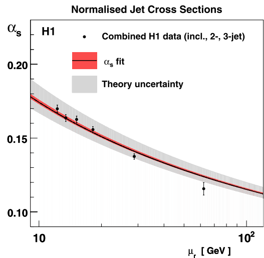
Fig. 12 The values of \alpha_s(\mu_r) obtained by a simultaneous fit of all normalised jet cross sections in each Q^2 bin. The solid line shows the two loop solution of the renormalisation group equation obtained by evolving the \alpha_s extracted from a simultaneous fit of 54 measurements of the normalised inclusive jet cross section as a function of Q^2 and P_T , the normalised 2-jet cross section as function of Q^2 and P_T and the normalised 3-jet cross section as function of Q^2 . Other details are given in the caption to Fig. 7
