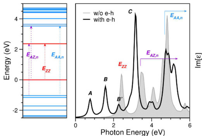
Fig. 3. Left: GW-corrected energy level scheme of (7,10)-AGNR. Tamm states are displayed in red, while bulk-like states are in blue. Right: Optical absorption spectrum of (7,10)-AGNR. The independent particle spectrum is in grey (shaded area), whereas the spectrum including e-h interaction at the BSE level is reported in black.
