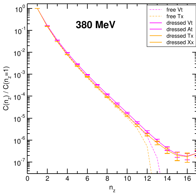
Fig. 3 Correlators of the V_t, A_t, T_x, X_x operators in full QCD at T=380 MeV ( \sim 2.2T_c ) for 32^3 \times 8 lattice (abbreviated as dressed ) and with non-interacting quarks ( free ) on the same lattice. From Ref. [6]
