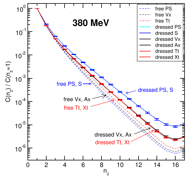
Fig. 5 Correlators of the PS, S, V_x, A_x, T_t, X_t operators in full QCD at T=380 MeV ( \sim 2.2T_c ) for 32^3 \times 8 lattice (abbreviated as dressed ) and with non-interacting quarks ( free ) on the same lattice. From Ref. [6]
