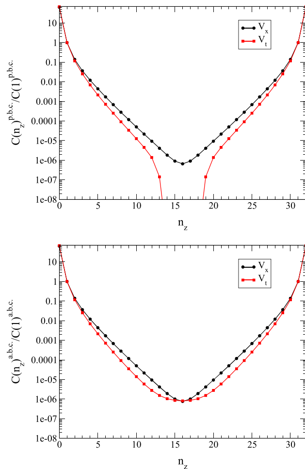
Fig. 2 Correlators of the V_t and V_x bilinears on a 32^3 \times 8 lattice with the overlap action with periodic (p.b.c., left panel) and antiperiodic (a.b.c., right panel) boundary conditions in z direction. The V_t correlator in the left panel is negative for n_z \sim 14 - 18 . The correlators are normalized to 1 at n_z = 1
