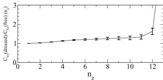
Fig. 4 Ratio of correlator of V_t operator in full QCD at T=380 MeV ( \sim 2.2T_c ) for 32^3 \times 8 lattice (abbreviated as dressed ) to V_t correlator calculated with non-interacting quarks on the same lattice size ( free )
