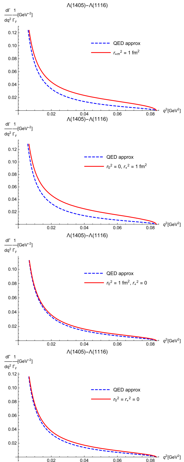
Fig. 1 Comparison between radius structure and QED-type approximation for the \frac{1}{2}^- \rightarrow \frac{1}{2}^+ transition. Top panel : both radii at maximal value (43); middle panels : one radius at max, one zero; bottom panel : both radii put to zero
