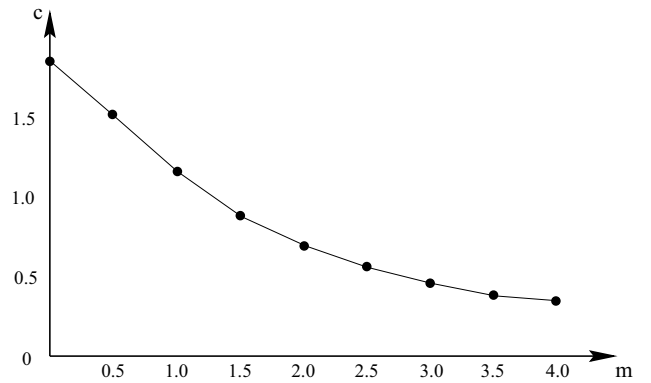
Fig. 18. A plot of the condensate parameter c vs. quark mass m for the regular solutions of the equation of motion in the Constable-Myers background. c and m are given in units set by the length scale b . From [18].
