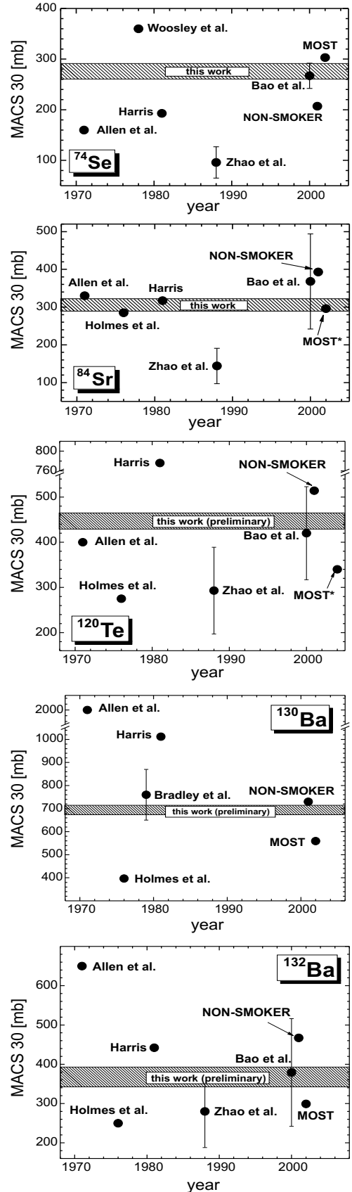
Fig. 1. Comparison of MACS30 predictions. MOST* marks modified values [20].
