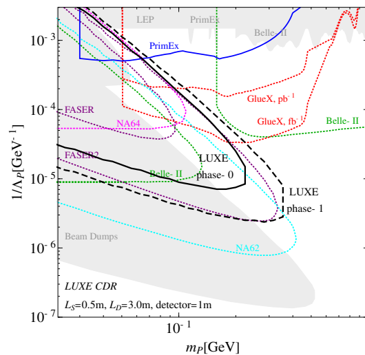
Fig. 6 Expected 95% confidence level sensitivity to ALPs for the LUXE experiment in phase-0 and phase-1 for one year of data taking in the plane of the ALP mass, m_P versus the coupling parameter 1/\Lambda_P . The grey area shows excluded areas based on LEP [22–24], PRIMEX [25], NA64 [26, 27], Belle-II [28], and beam-dumps experiments [29, 30]. In addition, projected sensitivities of future experiment are shown: NA62, Belle-II, FASER, PRIMEX and GLUEX [25, 31–34]
