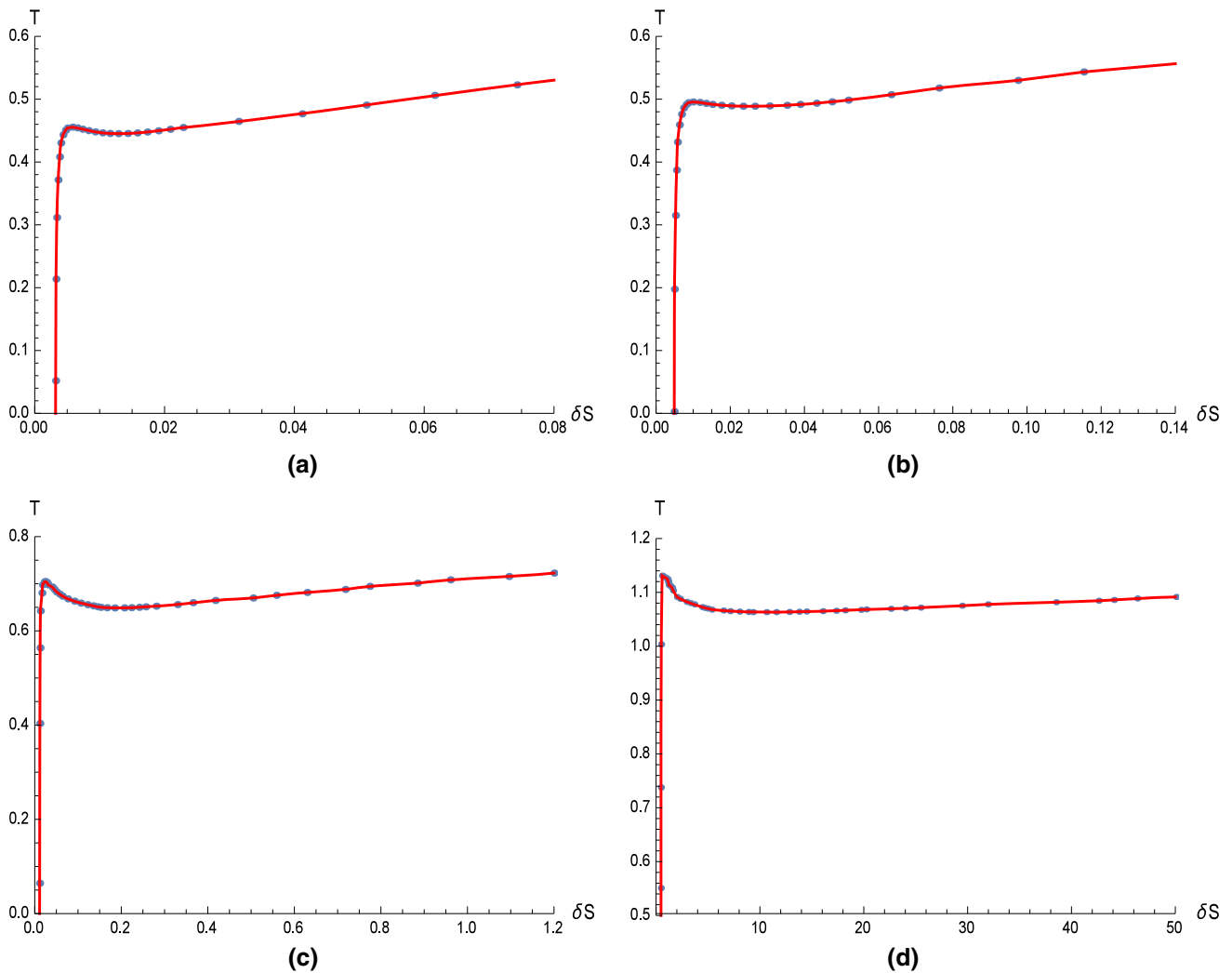
Fig. 10 T vs. \delta S for n = 4, \theta_0 = 0.3 . a \alpha = 0, q = 0.12 , b \alpha = 0.25, q = 0.12 , c \alpha = 0.5, q = 0.06 , d \alpha = 0.75, q = 0.06
