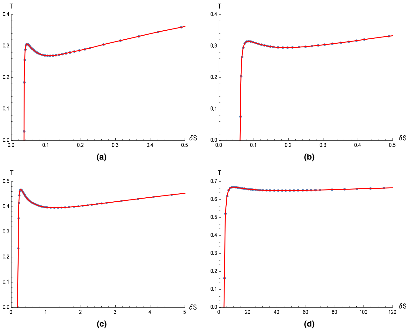
Fig. 9 T vs. \delta S for n = 3, \theta_0 = 0.3 . a \alpha = 0, q = 0.12 , b \alpha = 0.25, q = 0.12 , c \alpha = 0.5, q = 0.06 , d \alpha = 0.75, q = 0.06
