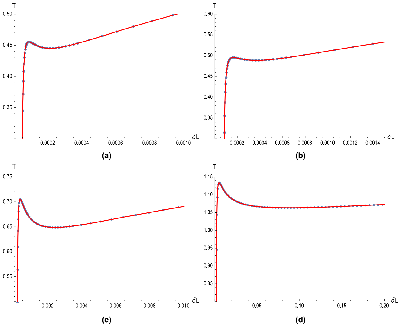
Fig. 2 T vs. \delta L for n = 4, \theta_0 = 0.2 . a \alpha = 0, q = 0.12 , b \alpha = 0.25, q = 0.12 , c \alpha = 0.5, q = 0.06 , d \alpha = 0.75, q = 0.06
