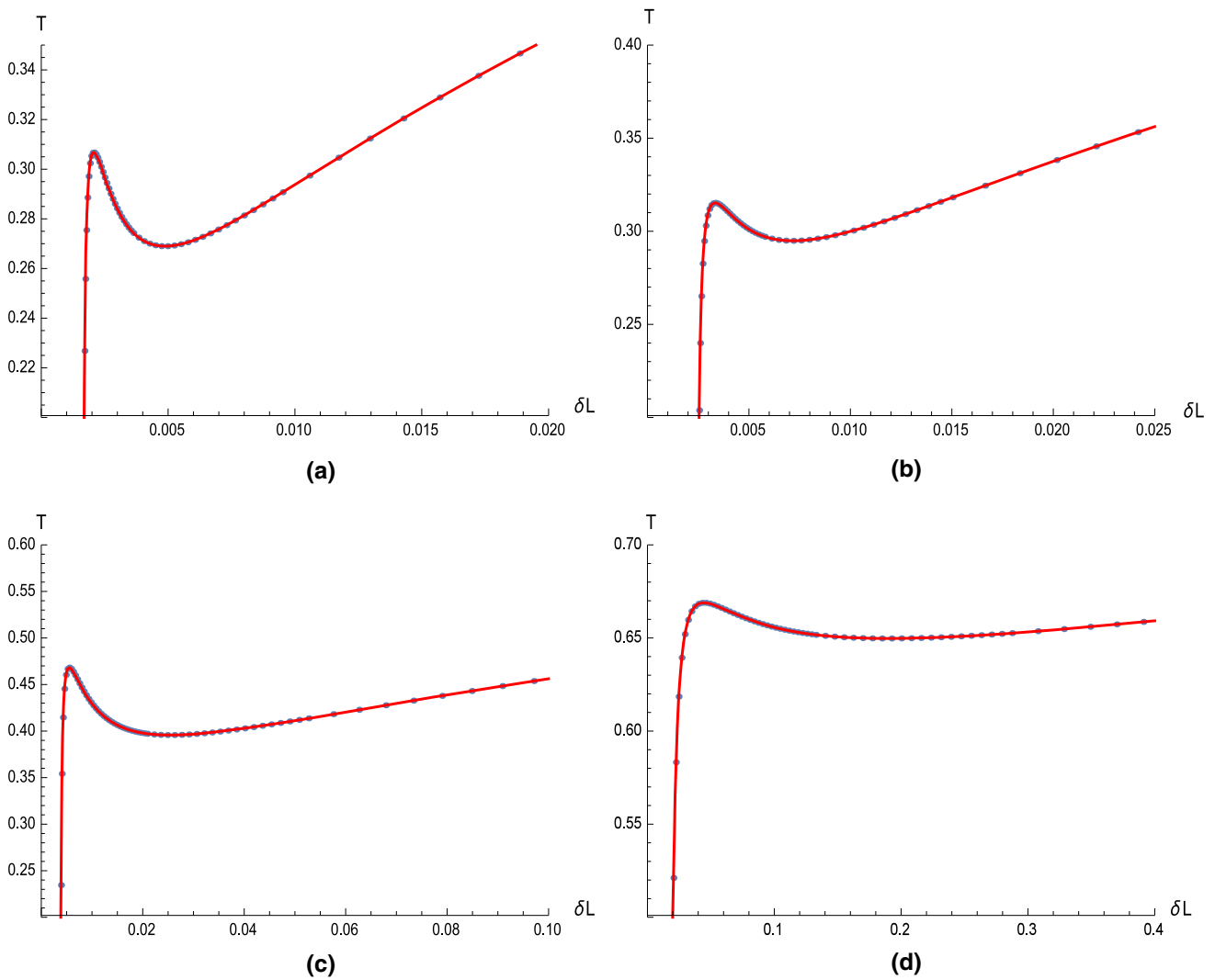
Fig. 3 T vs. \delta L for n = 3, \theta_0 = 0.3 . a \alpha = 0, q = 0.12 , b \alpha = 0.25, q = 0.12 , c \alpha = 0.5, q = 0.06 , d \alpha = 0.75, q = 0.06
