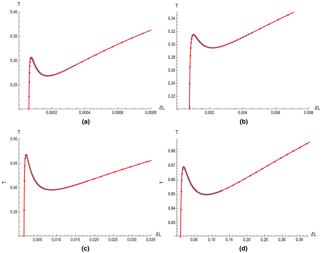
Fig. 1 T vs. \delta L for n = 3, \theta_0 = 0.2 . a \alpha = 0, q = 0.12 , b \alpha = 0.25, q = 0.12 , c \alpha = 0.5, q = 0.06 , d \alpha = 0.75, q = 0.06
