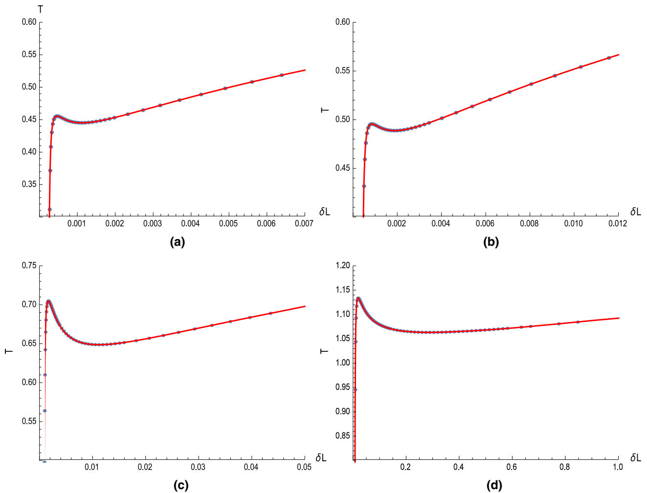
Fig. 4 T vs. \delta L for n = 4, \theta_0 = 0.3 . a \alpha = 0, q = 0.12 , b \alpha = 0.25, q = 0.12 , c \alpha = 0.5, q = 0.06 , d \alpha = 0.75, q = 0.06
