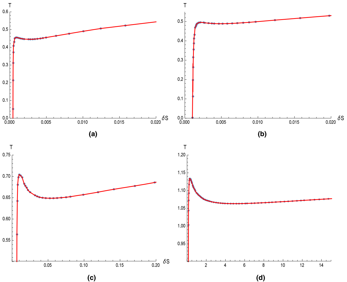
Fig. 8 T vs. \delta S for n = 4, \theta_0 = 0.2 . a \alpha = 0, q = 0.12 , b \alpha = 0.25, q = 0.12 , c \alpha = 0.5, q = 0.06 , d \alpha = 0.75, q = 0.06
