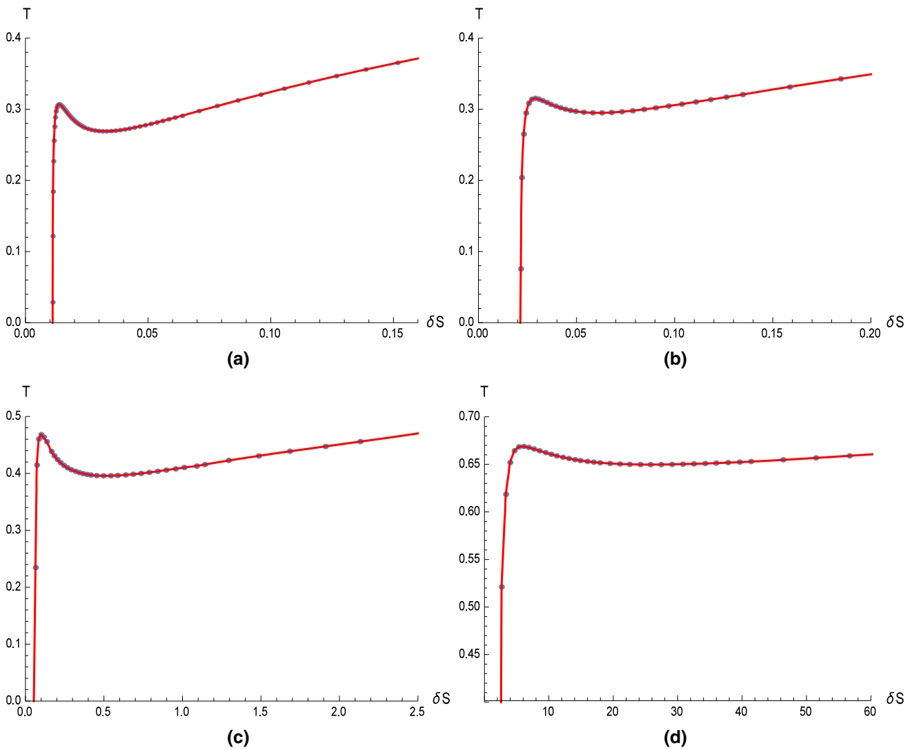
Fig. 7 T vs. \delta S for n = 3, \theta_0 = 0.2 . a \alpha = 0, q = 0.12 , b \alpha = 0.25, q = 0.12 , c \alpha = 0.5, q = 0.06 , d \alpha = 0.75, q = 0.06
