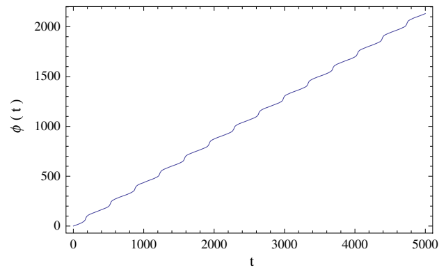
Fig. 25 Late time variation of \phi(t) in Model II for C = 0.5 and m = 20
