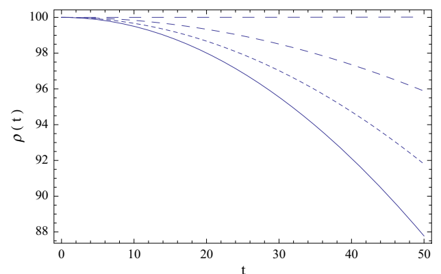
Fig. 17 Time variation of \rho(t) in Model II for m = 1 and different values of \dot{\theta}_0^2 : \dot{\theta}_0^2 = 0 (solid curve), \dot{\theta}_0^2 = 1/6 (dotted curve), \dot{\theta}_0^2 = 1/3 (short dashed curve) and \dot{\theta}_0^2 = 1/2 (long dashed curve)
