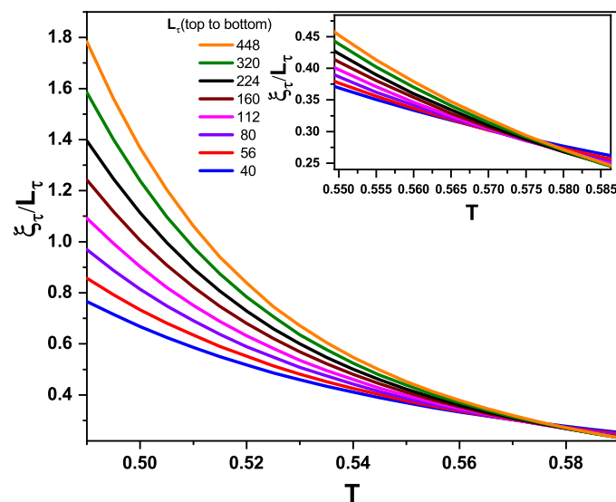
Fig. 9. Scaled correlation time \xi_\tau/L_\tau versus temperature T for different values of L_\tau in the Griffiths region. The system size in space is L = 1000 ; the data are averaged over 2000 disorder configurations. The inset shows a magnification for the crossing point of the curves.
