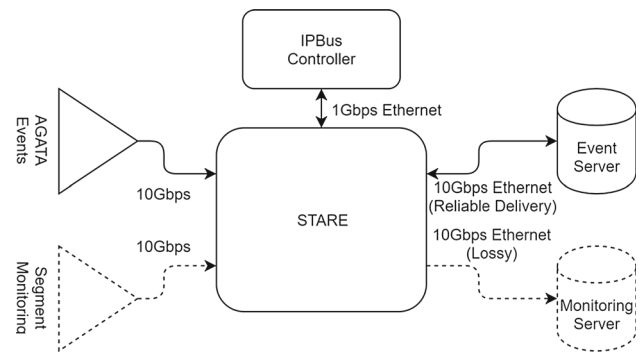
Fig. 12 The STARE conceptual design
