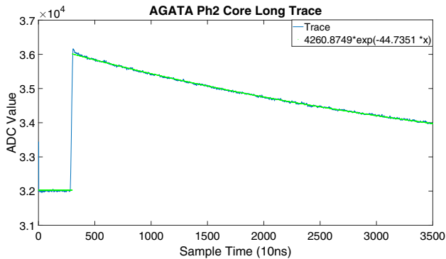
Fig. 11 First PACE readout of a 35 \mu s AGATA core signal trace with the fit of the pre-amplifier response function
