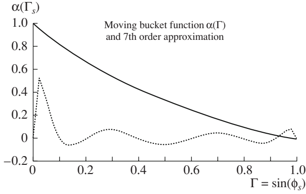
Fig. 10. Moving bucket function \alpha(\Gamma_s) and error in percent.
