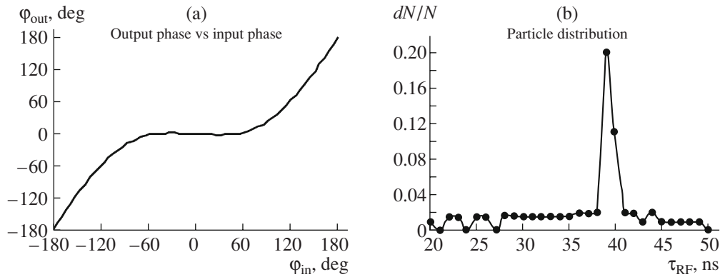
Fig. 3. Beam pulses at an RF frequency of f_{\text{RF}} = 10 MHz. The buncher voltage of 715 V was selected to focus the beam on the reaction microscope. The minimum available pulse width is \tau = 2 ns.
