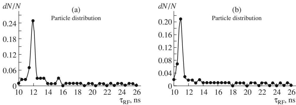
Fig. 6. Assumed effective field length of 25 mm (a) and 30 mm (b) at f_{RF} = 20 MHz. Buncher voltages are 390 and 380 V, respectively, with L_{drift} = 2.0 m and a pulse duration of at least 1.5 ns.
