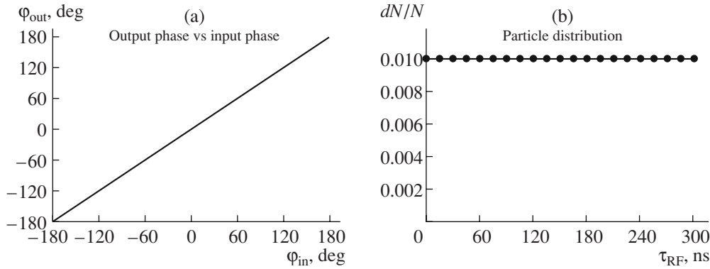
Fig. 1. Buncher_U400 code output with zero voltage on the buncher. (a) \phi_{\text{out}} as a function of \phi_{\text{in}} ; (b) intensity distribution vs RF phase: dN/N = f(\phi_{\text{in}}) .
