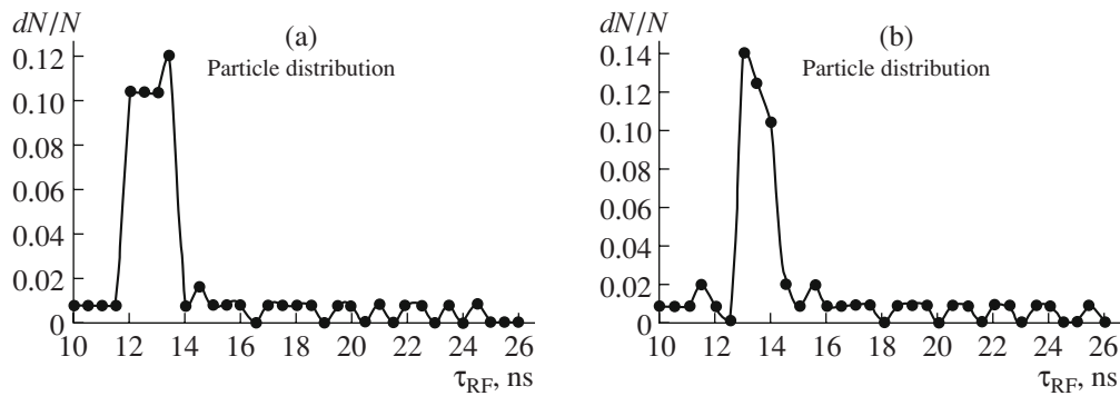
Fig. 7. Bunching of beam with momentum deviation of dp/p = -4\% (a) and dp/p = -0.15\% (b). Pulse width is 2.2 and 2 ns, respectively.
