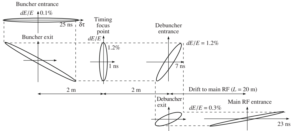
Fig. 9. Sketch of the evolution of the phase space ellipses in the short pulse operation mode.
