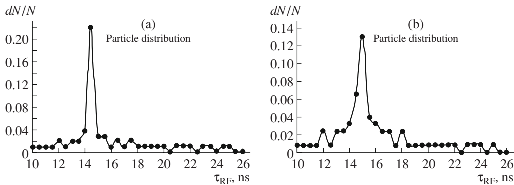
Fig. 8. Bunching of beam with momentum deviation of dp/p = 2.5\% (a) and dp/p = 4\% (b). Pulse width is 1.3 and 1.7 ns, respectively.
