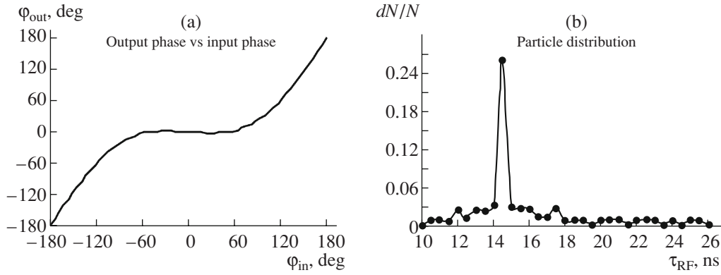
Fig. 5. Beam pulses at an RF frequency of f_{RF} = 20 MHz. The amplitude of the buncher voltage is V = 370 V and is optimized to focus the beam pulse on the reaction microscope after a drift of L_{drift} = 2.0 m. The width of the gap is d_{gap} = 20 mm and the pulse width is \tau = 1 ns.
