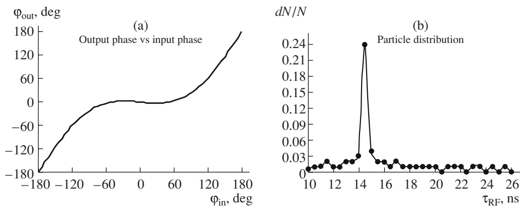
Fig. 4. Beam pulses at an RF frequency of f_{\text{RF}} = 20 MHz. The amplitude of the buncher voltage is V = 515 V and is optimized to focus the beam pulse on the reaction microscope after a drift of L_{\text{drift}} = 1.4 m. The width of the gap is d_{\text{gap}} = 20 mm and the pulse width is \tau = 1 ns.
