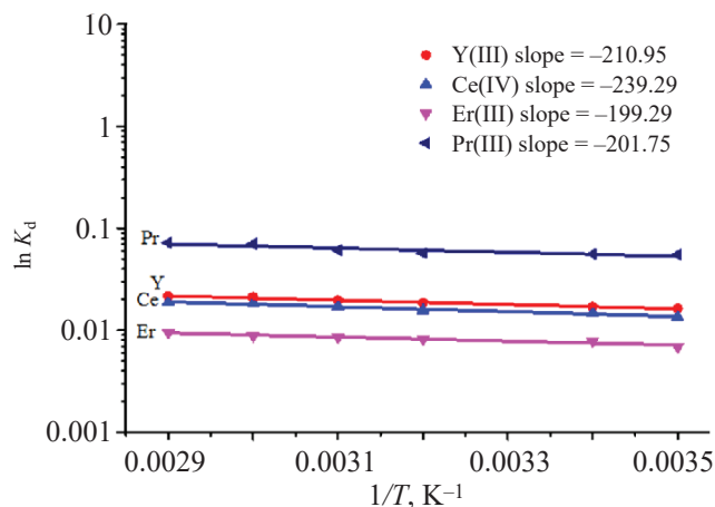
Fig. 4. Relation between (\ln K_d) and (1/T) on the sorption of REEs from phosphate medium onto SQS-6 resin.
