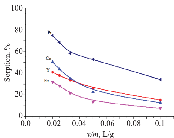
Fig. 3. Effect of v/m ratio on the sorption of REEs (200 mg/L each) on SQS-6 resin from 8.0 M phosphoric acid.
