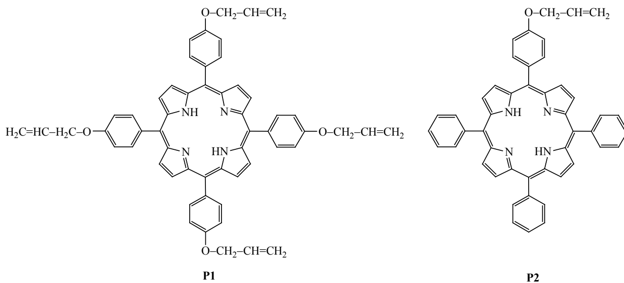
Fig. 1. Structural formulas of the porphyrin monomers P1 and P2.
