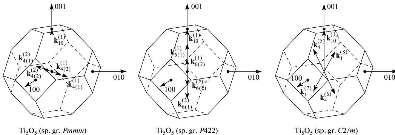
Fig. 2. Superstructure vectors of the reciprocal lattices of the orthorhombic (space group Pmmm ), tetragonal (space group P422 ), and monoclinic (space group C2/m ) super structures of type \text{Ti}_5\text{O}_5 , which enter in the channels of disorder–order ( \text{Ti}_x\text{O}_z – \text{Ti}_5\text{O}_5 ) phase transitions and their location in the first Brillouin zone of the fcc lattice.
