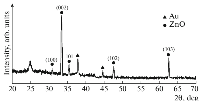
Fig. 6. XRD pattern of grown ZnO nanowires at 1.0 V, perpendicular to the growth direction.
