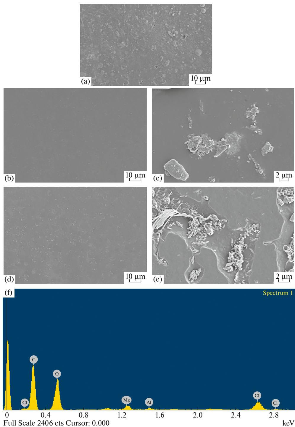
Fig. 2. (a–e) SEM and (f) EDS analysis of polymer electrolyte films for different wt% ratios of PVP: (a) pure PVP, (b) (95 : 5), (c) (90 : 10), (d) (85 : 15), (e) (80 : 20).
