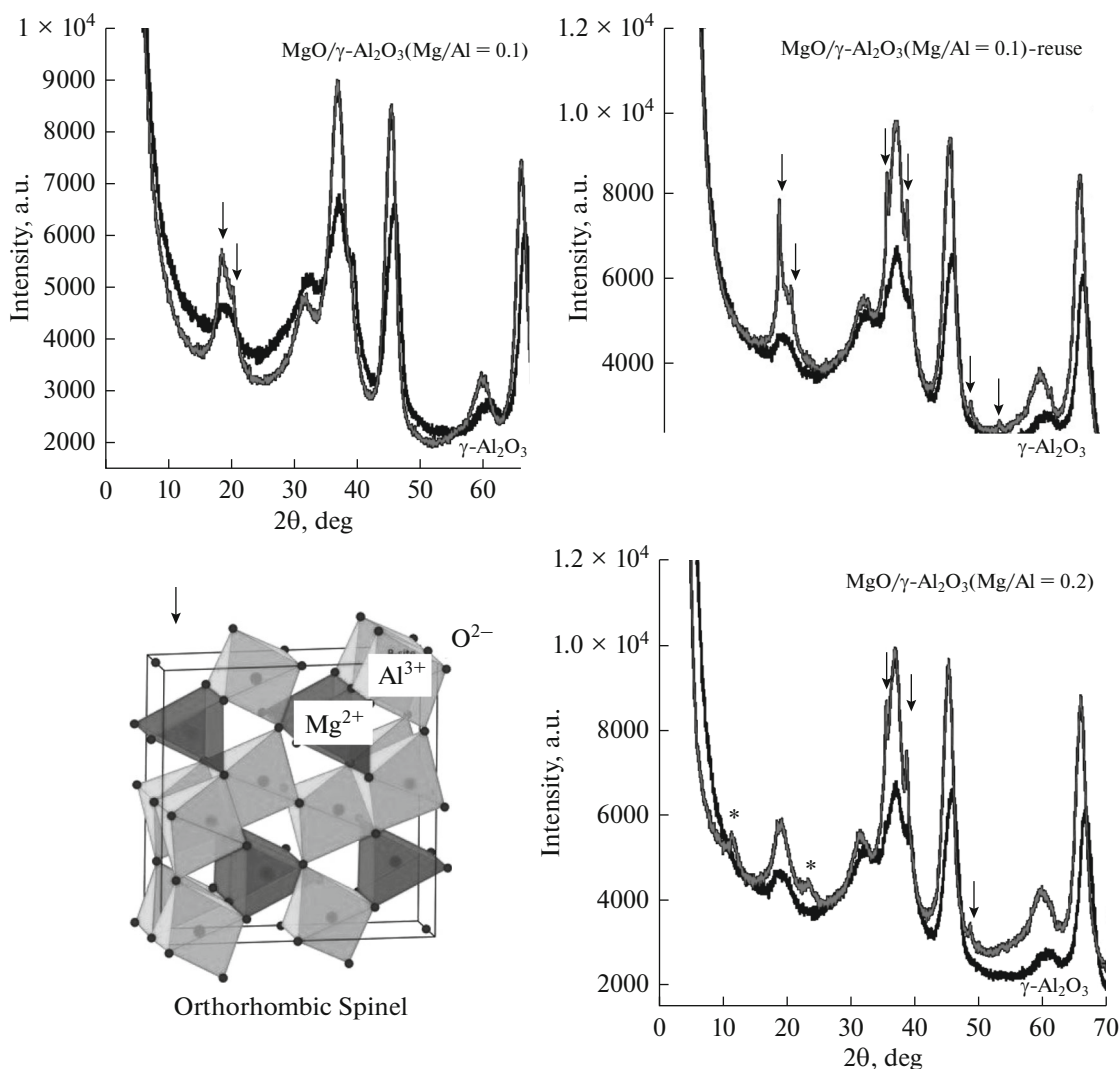
Fig. 13. XRD pattern of catalysts after catalytic ozonation: (grey) \text{Mg}/\gamma\text{-Al}_2\text{O}_3 ( \text{Mg}/\text{Al} = 0.1 ) after 1 and 2 ozonations (reuse) and \text{Mg}/\gamma\text{-Al}_2\text{O}_3 ( \text{Mg}/\text{Al} = 0.2 ) after 1 ozonation. For comparison in each graph (black) calcined \gamma\text{-Al}_2\text{O}_3 ( 600^\circ\text{C} ) after 1 ozonation. Diffraction peak for orthorhombic spinel (arrows) and LDH – d_{100} = 0.78 nm (*). Schematic representation of the orthorhombic spinel structure.
