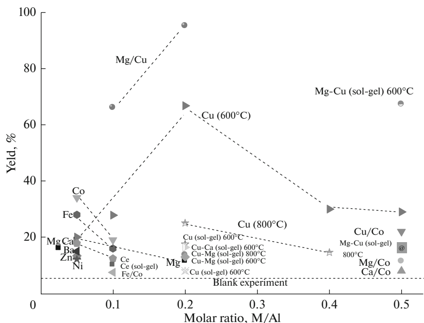
Fig. 5. Oxidation test: yields of benzaldehyde with the different M/Al 2 O 3 catalysts. The reaction condition: benzyl alcohol (517 \mu L), cyclohexane (15 mL), 0.3 g catalyst, 150°C for 24 h, under air 2.0 bar.
