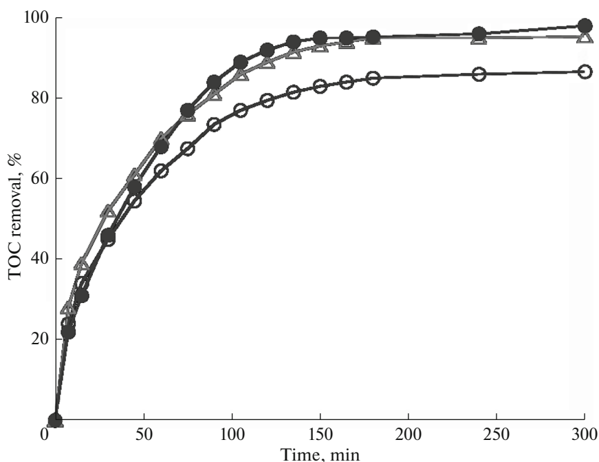
Fig. 7. TOC removal (%) of saline petroleum effluents (initial TOC = 216 mg/L) as a function of ozonation time for Mg/ \gamma -Al 2 O 3 (Mg/Al = 0.1) calcined at 600°C with (○) 3.3 and (△) 5 g/L of catalyst and (●) in reuse with 3.3 g/L of catalyst.
