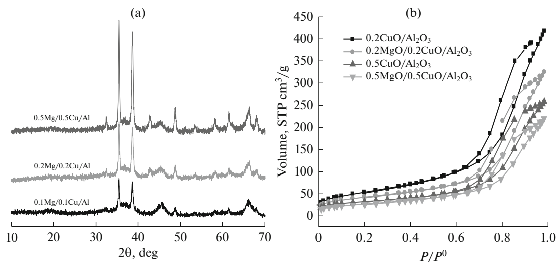
Fig. 3. (a) XRD patterns and nitrogen sorption isotherms at 77 K of Mg/Cu/ \gamma -Al 2 O 3 samples prepared by incipient wetness impregnation with different molar ratios and calcined at 600°C.
