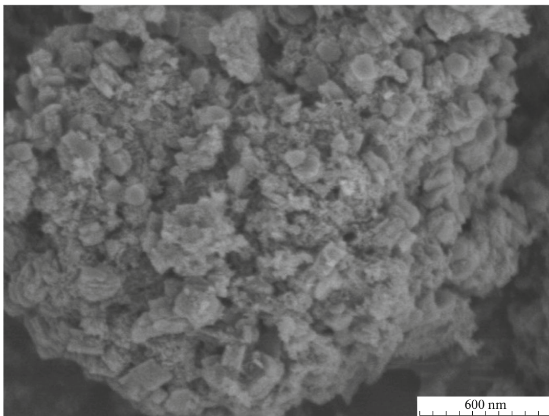
Fig. 8. SEM pictures of Mg/γ-Al 2 O 3 (Mg/Al = 0.1) after two catalytic ozonations.
