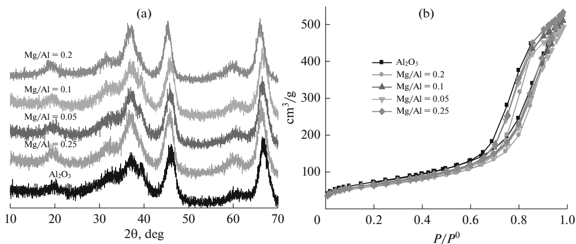
Fig. 1. (a) XRD patterns and (b) nitrogen sorption isotherms at 77 K of \gamma -Al 2 O 3 and Mg/ \gamma -Al 2 O 3 samples prepared by incipient wetness impregnation with different Mg/Al molar ratios and calcined at 600°C.
