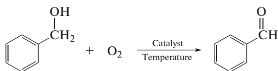
Scheme 1. Catalytic oxidation of benzyl alcohol to benzaldehyde.
