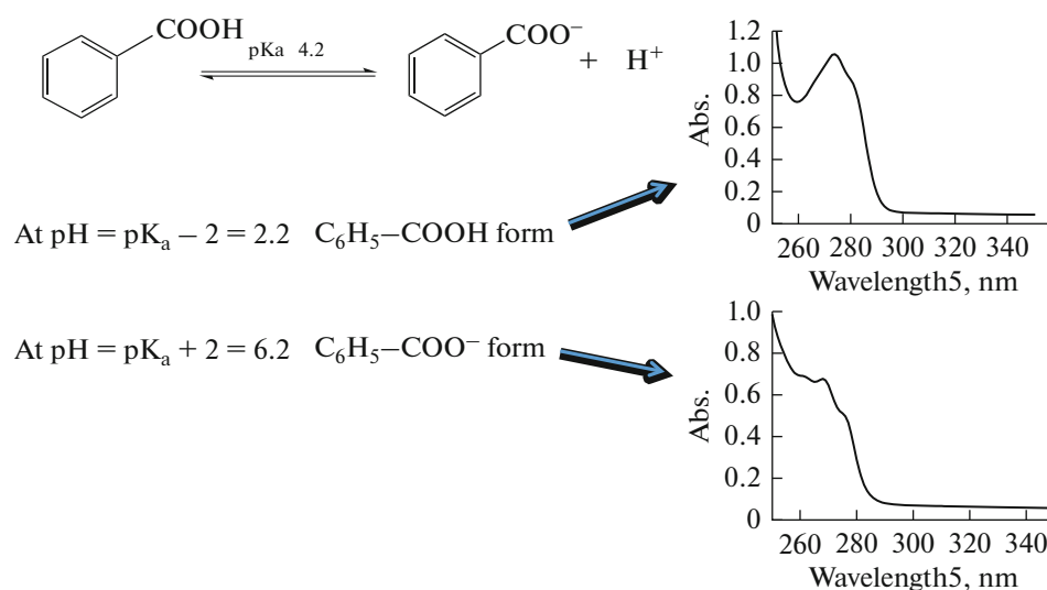
Scheme 2. Example of UV spectra of benzoic acid obtained in acidic and basic conditions.
