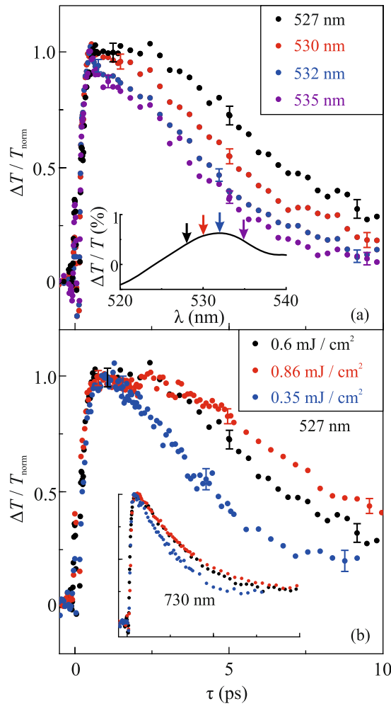
Fig. 3. (Color online) (a) \Delta T/T(\tau) cross sections for several wavelengths near the QWG normalized on the maximum value; the inset: \Delta T/T(\lambda) spectrum near the QWG and arrows indicating considered wavelengths. (b) Normalized \Delta T/T(\tau) cross sections at 527 nm wavelength for several fluences; the inset shows normalized \Delta T/T(\tau) cross sections at 730 nm wavelength for the same fluences.
