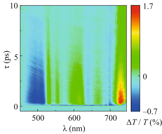
Fig. 1. (Color online) Differential transmittance \Delta T/T dependence on the wavelength \lambda and time delay \tau .
