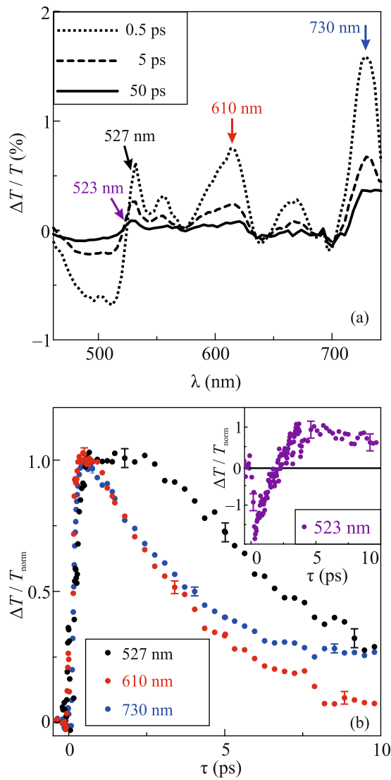
Fig. 2. (Color online) (a) Cross sections of differential transmittance \Delta T/T(\lambda) for different delay times. (b) \Delta T/T(\tau) cross sections for different wavelengths normalized on maximum, the wavelengths are marked with arrows in the panel (a); the inset shows the cross section at 523 nm near zero value of \Delta T/T .
