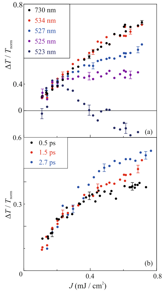
Fig. 4. (Color online) (a) \Delta T/T(J) dependence normalized on linear part in the vicinity of dipole SLR (black dots) and QWG for several wavelengths. (b) \Delta T/T(J) dependence normalized on linear part for different delay times in the vicinity of QWG at 527 nm wavelength.
