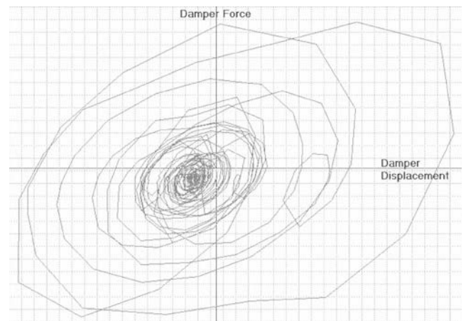
Fig. 2: Force vs. displacement during seismic event on February 28, 2001
