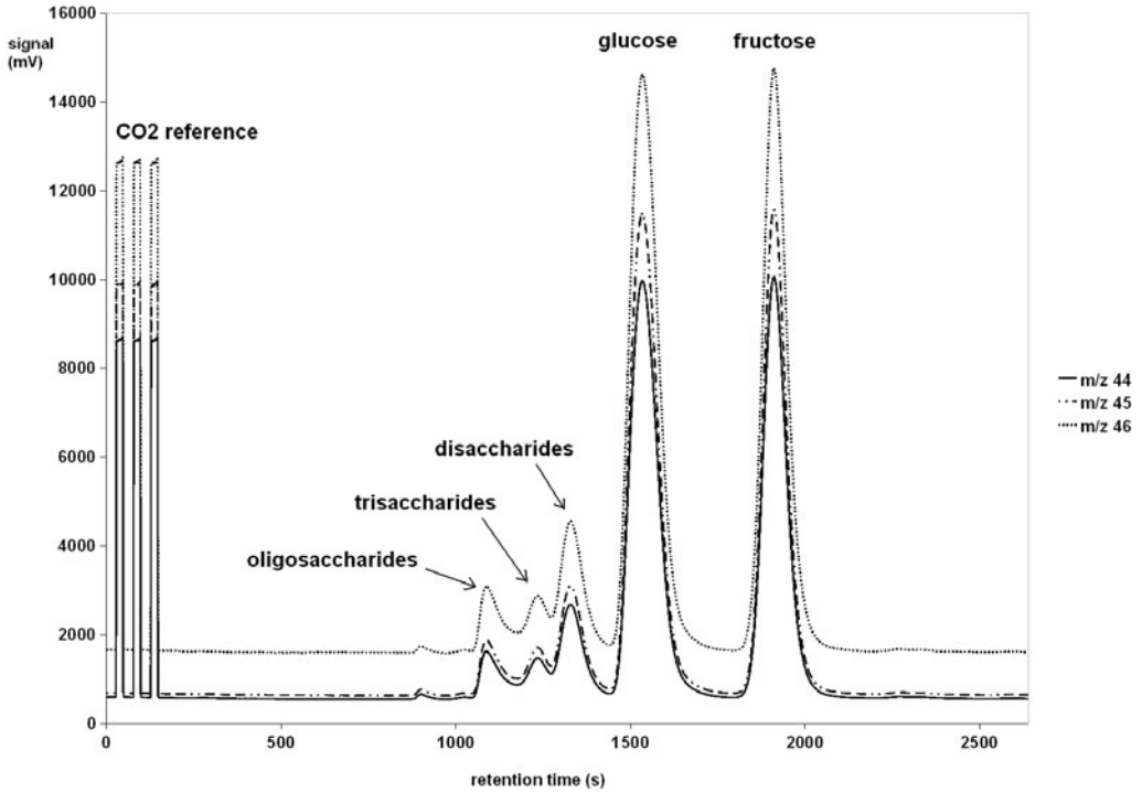
Figure 2. LC-IRMS chromatogram of adulterated polyfloral honey (sample 2d, Table VII). \delta^{13}\text{C} values: fructose -27.4\text{‰} , glucose -27.0\text{‰} , disaccharides -26.4\text{‰} , trisaccharides -24.3\text{‰} , oligosaccharides -26.7\text{‰} . Adulteration: ca. 11% rice syrup.
