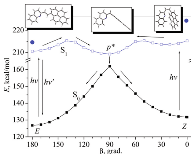
Fig. 6 Minimal energy paths of the isomerization reaction of the 1P2QE s-cis -conformer in the S_0 state (calculated by the PM3 method) and in the S_1 state (calculated by the PM3-CI(2 × 2) method); the arrows show the diabatic reaction path. The filled circles mark the location of the terms of the vertically excited isomers.
