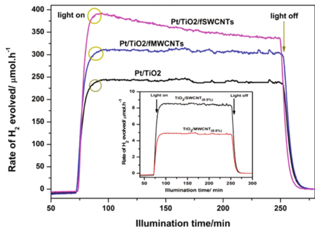
Fig. 8 Timeline of nanocomposite photocatalytic H 2 evolution from methanol aqueous solution (timeline of photocatalytic H 2 evolution from methanol aqueous solution in the presence of TiO 2 /fCNTs (fSWCNTs, fMWCNTs). Experimental conditions: methanol conc. 5 mM, light intensity 40 mW cm -2 , mass of catalyst 50 mg, and irradiation time 3 h.
