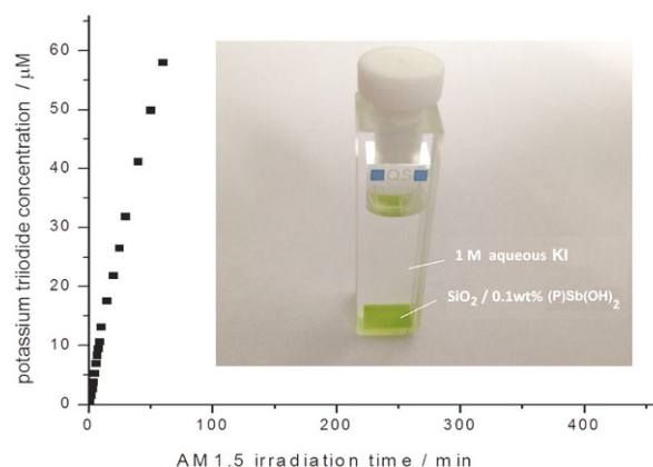
Fig. 6 Initial rate of solar photocatalytic triiodide formation and picture of a freshly prepared sample cuvette before exposure to simulated sunlight with t = 0\text{--}60 min irradiation times under AM 1.5 conditions. All concentrations are such as those reported in Fig. 5.
