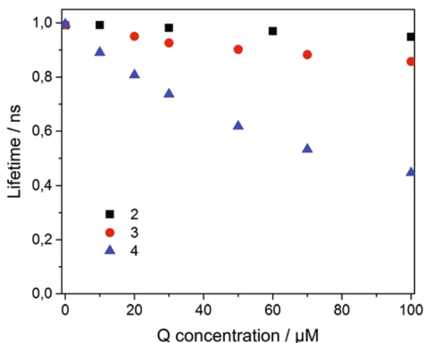
Fig. 4 Fluorescence lifetime ( \lambda_{\text{exc}} = 375 \text{ nm} ) of 1 incorporated into \beta -CDV in phosphate buffer (pH 7.2) dependent on the concentration of the quencher ( Q ) 2 (black square), 3 (red circle) and 4 (blue triangle).
