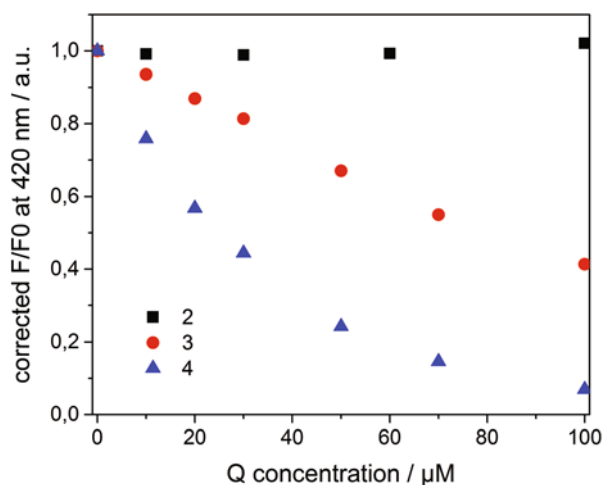
Fig. 3 F/F_0 at 420 \text{ nm} ( \lambda_{\text{exc}} = 375 \text{ nm} ) of 1 incorporated into \beta -CDV in phosphate buffer (pH 7.2) as a function of the concentration of the quencher ( Q ) 2 , 3 and 4 . F and F_0 are the emission maxima in the presence and absence of quenchers, respectively.
