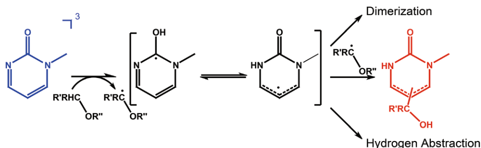
Fig. 5 Scheme summarizing HA by ^3\text{1MP}^* . 1MP in the triplet state abstracts a hydrogen atom from the quencher bearing a -\text{CRH}-\text{O}- chemical motif. The so formed radical can tautomerize forming a NH group. Recombination with the quencher radical terminates the reaction chain. For high concentrations also dimerization could occur.
