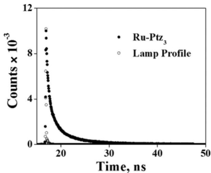
Fig. 4 Emission decay profile of Ru-Ptz 3 in ACN. Excitation was at 401 nm and emission was monitored at 630 nm. The lamp profile is also shown.
