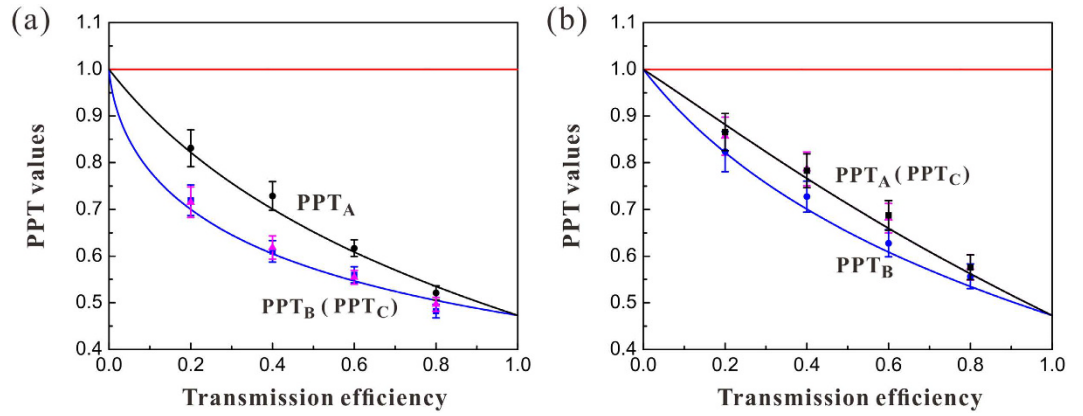
Figure 2. The entanglement in lossy channels. (a) One optical mode \hat{A} is distributed in the lossy channel ( \eta_A \neq 1, \eta_C = 1 ). (b) Two optical modes \hat{A} and \hat{C} are distributed in the lossy channels with the same transmission efficiency ( \eta_A \neq 1, \eta_C \neq 1 ). PPT values are all below the entanglement boundary (red lines), which means that the tripartite entanglement is robust against loss in quantum channels. The black, blue and pink dots represent the experimental data for different PPT values, respectively. Error bars represent \pm one standard deviation and are obtained based on the statistics of the measured noise variances.
