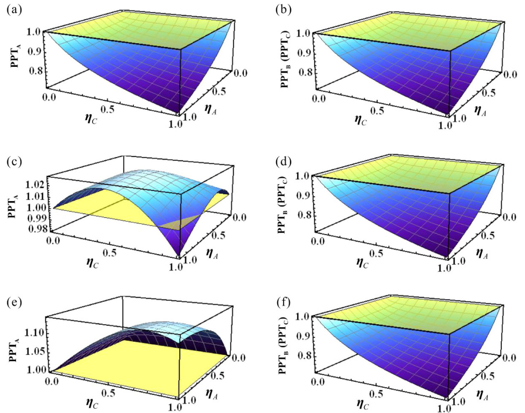
Figure 3. The entanglement properties of different asymmetric tripartite states in two lossy channels. (a,b) PPT values of fully robust entanglement against loss with c_x/c = 0.8 . (c,d) PPT values of a one-mode fragile state in lossy channels with attenuations with c_x/c = 0.5 . (e,f) A totally one-mode biseparable state in lossy channels with c_x/c = 0.3 .
