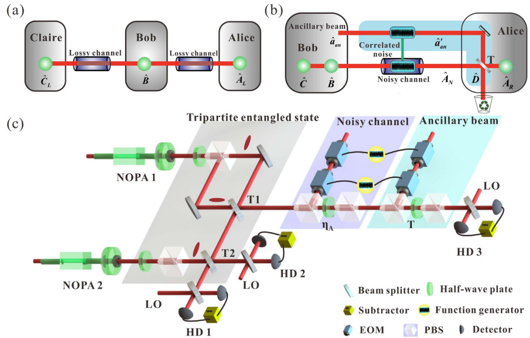
Figure 1. Schematic of principle and experimental set-up. (a) Two modes ( \hat{A} and \hat{C} ) of a tripartite entangled state are distributed over two lossy quantum channels to Alice and Claire, respectively. (b) One mode of the tripartite entangled state is distributed over a noisy channel, where disentanglement is observed among optical modes \hat{A}_N , \hat{B} and \hat{C} . The entanglement revival operation is implemented by coupling an ancillary beam ( \hat{a}'_{an} ) who has correlated noise with the environment with the transmitted mode \hat{A}_N on a beam-splitter with transmission efficiency of T , thus the entanglement among modes \hat{A}_R , \hat{B} and \hat{C} is revived. (c) The schematic of experimental set-up for distributing a mode of the tripartite entangled optical beams over a noisy channel and the entanglement revival. T1 and T2 are the beam-splitters used to generate the GHZ entangled state. \eta_A and T are the transmission efficiencies of the noisy channel and the revival beam-splitter, respectively. HD1-3, homodyne detectors. LO, the local oscillator.
