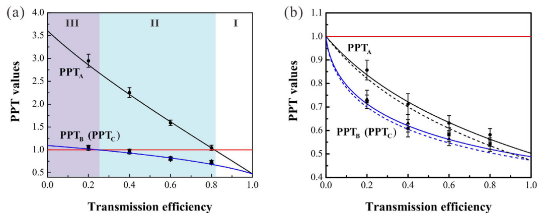
Figure 4. The disentanglement and entanglement revival in a noisy channel. (a) The PPT values for the transmission in a noisy channel, where the variance of the excess noise is taken as five times of shot noise level. The tripartite entangled state experiences entanglement (I), one-mode biseparable (II) and fully disentanglement (III) along with the decreasing of the channel efficiency. (b) The PPT values after entanglement revival. Dash lines are the corresponding results of the perfectly revival, the results are the same with the lines in Fig. 2(a) which are obtained before disentanglement. The black dots represent the experimental data. Error bars represent \pm one standard deviation and are obtained based on the statistics of the measured noise variances.
