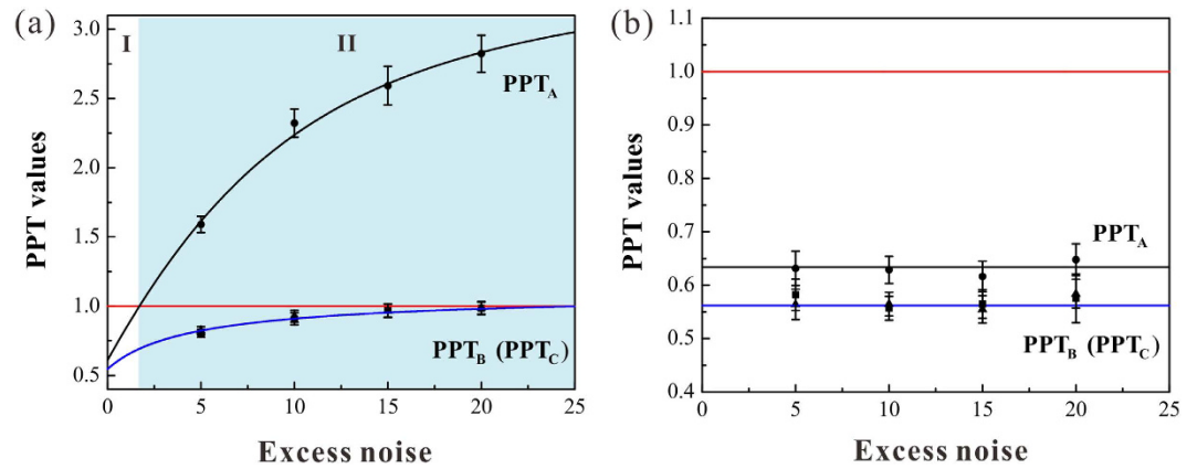
Figure 5. The disentanglement and revival of entanglement at different noise levels (in the unit of shot noise level). (a) Disentanglement at different excess noise levels. (b) The PPT values after entanglement revival, and it is independent on the excess noise. The black dots represent the experimental data. Error bars represent \pm one standard deviation and are obtained based on the statistics of the measured noise variances.
