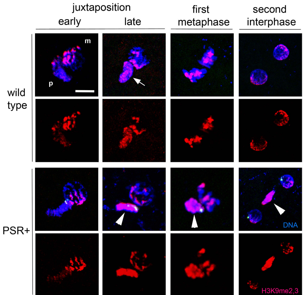
Figure 3. PSR disrupts histone H3K9me2 and H3K9me3 patterns on paternally-derived chromatin. In wild type embryos H3K9me2,3 begins to appear in localized regions of the paternal chromatin following juxtaposition. The signal persists in these regions while increasing in intensity (white arrow) until they are similar to regions on the maternal chromatin. This mark persists during metaphase, and obtains a RABL-like confirmation in the pericentromeric regions on opposing sides of the two daughter nuclei at the end of the first mitosis. In PSR-carrying embryos, the paternal chromatin obtains abnormally high levels of H3K9me2,3 across its entirety instead of in distinct regions (white arrowheads). This pattern persists following the end of the first mitosis. Scale bar is 10 \mu M.
