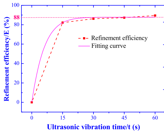
Figure 11. Grain refinement efficiency under different ultrasonic vibration time.
