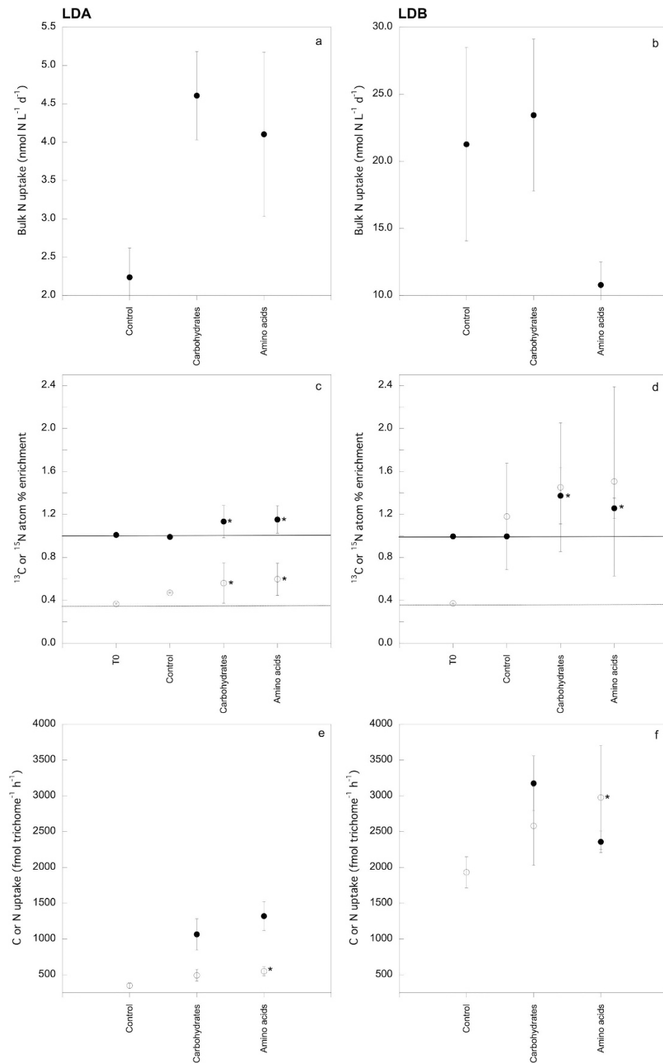
Figure 1. Bulk seawater N uptake rates at (a) station LDA, and (b) station LDB (note the different scale ranges on the y-axis). Trichodesmium (c,d) 13 C -filled circles- and 15 N -open circles- atom % enrichment values, and (e,f) 13 C and 15 N uptake rates at stations LDA and LDB, respectively. Error bars for C or N uptake rates (a,b,e,f) represent the standard error, while error bars for atom % graphs (c,d) represent the standard deviation of the mean. Straight and dotted lines in (c,d) indicate the average 13 C and 15 N atom % enrichment, respectively, of time zero samples (average natural abundance). Asterisks indicate statistically significant differences (Mann Whitney test, p < 0.05 ).
