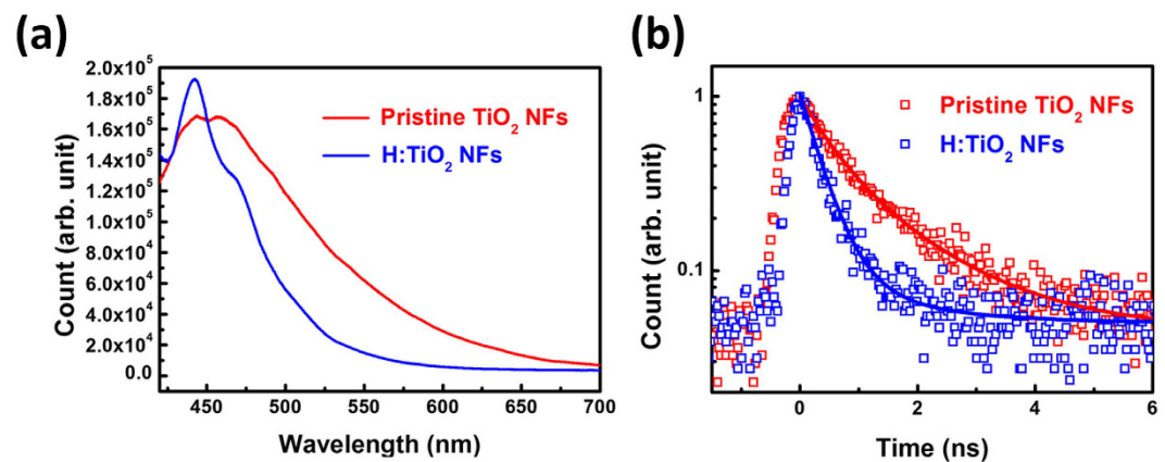
Figure 6. (a) PL spectra and (b) \mu -TRPL spectrum of pristine TiO 2 -650 NFs and H:TiO 2 -650 NFs excited by 375 nm picosecond pulse laser.
