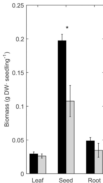
Figure 2. Mean dry Biomass (g) of leaves, seeds and roots of seedlings growing under high CO 2 (black) or control (grey) conditions. Error bars indicate standard error. Asterisk indicates statistically significant differences between treatments.
