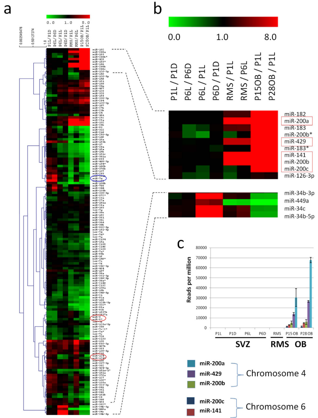
Figure 1. miRNome profiling by deep-sequencing. (a) Heatmap showing the results of deep sequencing analyses. Only microRNAs representing more than 0.1% of total microRNAs in at least one tissue are shown. Number of reads for a microRNA in a given tissue was obtained by averaging the different sample repetitions. Columns describe the ratios between tissues selected for comparison. Proximity of vertical position indicates the similarity of expression profile of detected microRNAs and was determined using the MeV application 60 . (b) Close-up of specific regions of the heat map highlighting the miR-200-family a group of microRNAs preferentially expressed in the OB and the miR-34 family that is induced during ciliogenesis. miR-34a does not cluster in the heatmap due to strong expression in OB glia. (c) Histogram representing the absolute number of reads per tissue obtained in the deep sequencing analysis for each member of the miR-200 family. All miR-200 family members are exclusively expressed in the OB but not in the stem cell or migratory compartments.
