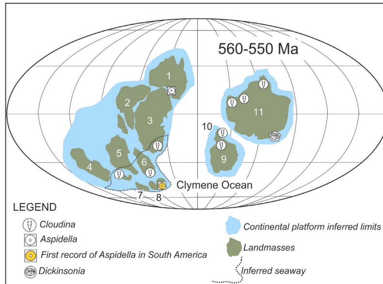
Figure 6. Schematic reconstruction of the Southeastern Gondwana paleogeography during the end of Ediacaran with fossil occurrences. 1-Australia, 2- India, 3-Antarctica, 4- West Africa, 5-Congo-São Francisco, 6- Kalahari, 7-Paraná, 8-Río de la Plata, 9-Amazônia, 10-Río Apa, 11-Laurentia (map made by L.V. Warren in Corel Draw X7 software).
