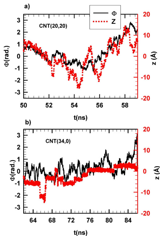
Figure 4. Time evolution of the azimuthal (black and left axis) and axial (red and right axis) coordinates of a single [\text{C}_4\text{mim}^+] cation confined in a) CNT(20,20) and b) CNT(34,0).
