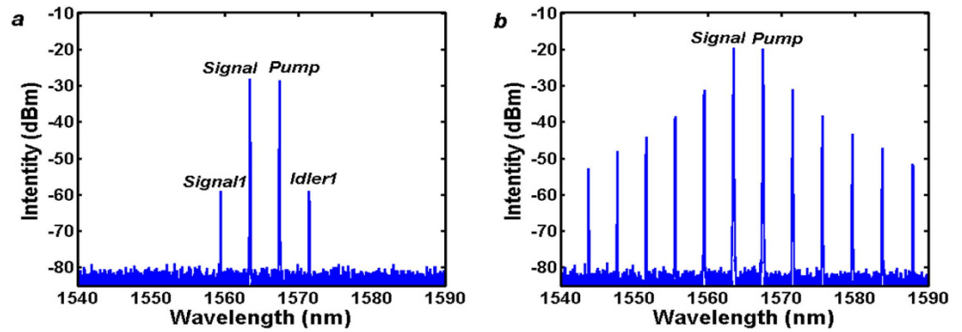
Figure 3. Experimental results for FWM in MRR with 490 GHz frequency spacing (10FSRs). (a) -1 dBm, (b) 10 dBm.
