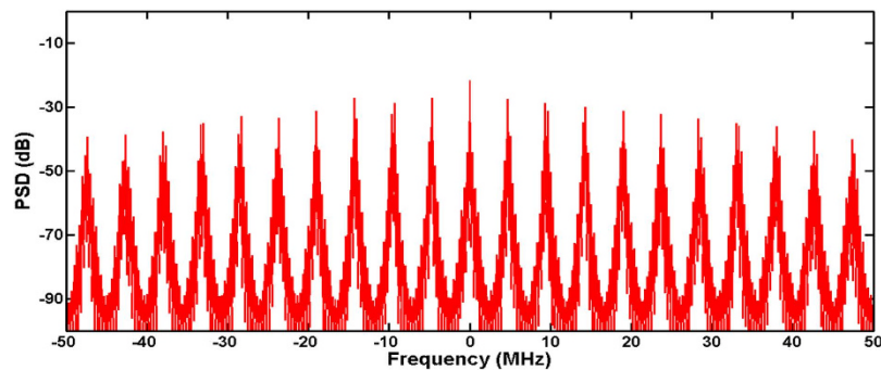
Figure 6. RF beating spectrum measured with a fast photo detector. PSD: Power Spectral Density.
