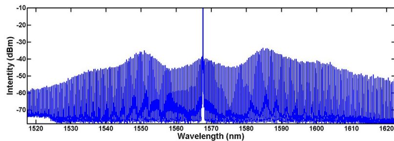
Figure 5. OFC spectrum generated by OPO in the MRR.
