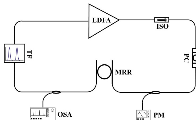
Figure 2. Experimental set-up for the self-locked tunable OFC generation. EDFA, erbium-doped fiber amplifier; ISO, Isolator; PC, Polarization Controller; MRR, Micro-Ring Resonator; TF, Tunable Filter; OSA, Optical Spectrum Analyzer; PM, Power Meter.
