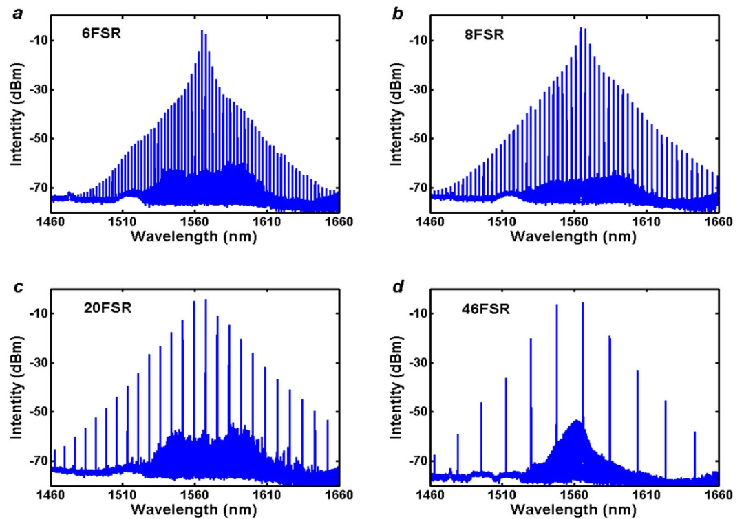
Figure 4. Spectra of generated OFC with different frequency spacing. (a) 6-FSR comb, (b) 8-FSR comb, (c) 20-FSR comb, (d) 46-FSR comb.
