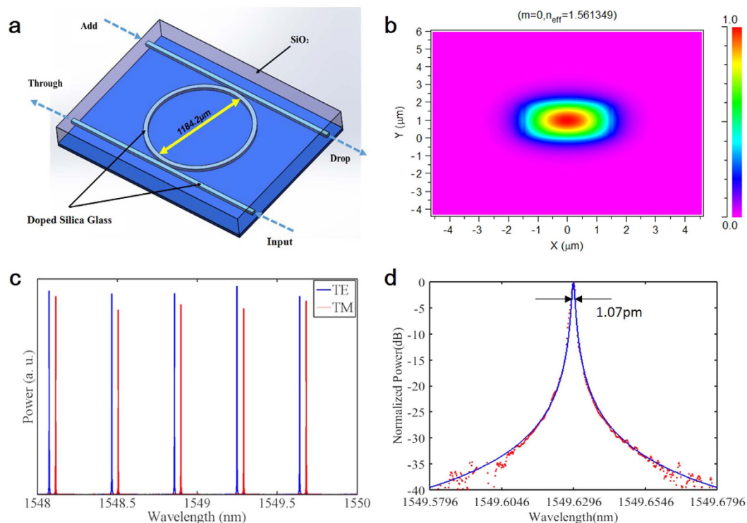
Figure 1. Device schematic and propagation characteristics. (a) Schematic of the four-port high-Q MRR. The waveguide core is a CMOS-compatible high-index doped silica glass. (b) Calculated mode profile for TE polarization. (c) Linear input-drop transmission characteristic of the ring resonator for TM and TE polarizations. (d) High-resolution resonance profile with a Lorentzian fit showing a 1.07 pm FWHM.
