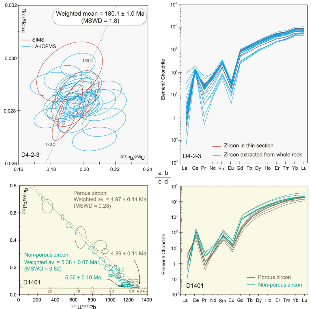
Figure 3. ^{207}\text{Pb} -corrected/ ^{230}\text{Th} -disequilibrium corrected ages for sample D4-2-3 (a–b) and D1401 (c–d).
