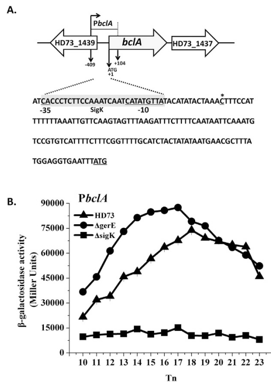
Figure 1. Nucleotide sequence and transcriptional activity of the bclA promoter. (A) Nucleotide sequence analysis. The indicated promoter region, 409 bp upstream and 104 bp downstream of the start codon (double-underlined), was fused with lacZ . Transcriptional start site (TSS, indicated by asterisks) is located 120 bp upstream from the start codon of the bclA gene. The SigK consensus sequence is indicated with a gray box, and the putative -35 and -10 sequences are underlined. (B) \beta -galactosidase activity assay of PbclA in wild-type HD73 (▲), sigK mutant (■), and gerE mutant (●). T_0 is the end of the exponential phase, and T_n is n hours after T_0 . Values represent mean of at least three independent replicates; error bars represent standard deviation.
