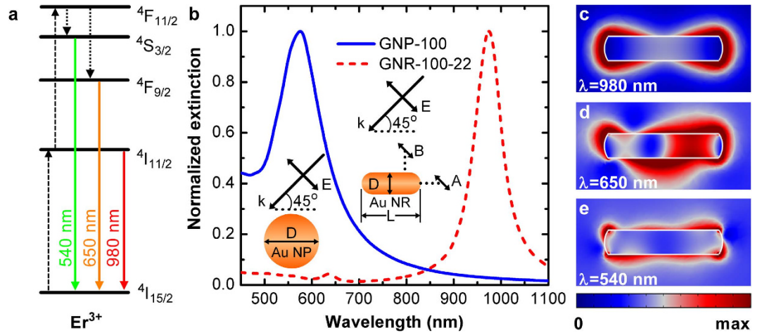
Figure 1. Simplified energy-level scheme of Er 3+ doped UCNCs and plasmonic properties of gold nanostructures. (a) Simplified energy-level scheme of Er 3+ doped UCNCs. Dashed, dotted and solid arrows indicate photon excitation, multi-phonon relaxation and emission processes, respectively. (b) Normalized extinction spectra of a gold nanoparticle with 100-nm diameter (blue curve) and a gold nanorod with 22-nm diameter and 100-nm length (red dashed curve). The insets in (b) show the excitation configuration for the gold nanoparticle and nanorod. Position A is on the longitudinal axis and position B is above the nanorod at a horizontal distance a quarter of the nanorod length to the nanorod end (c–e) Normalized E-field distribution in the GNR at wavelengths 980 (c), 650 (d), and 540 nm (e), corresponding to the excitation and emission wavelengths in (a).
