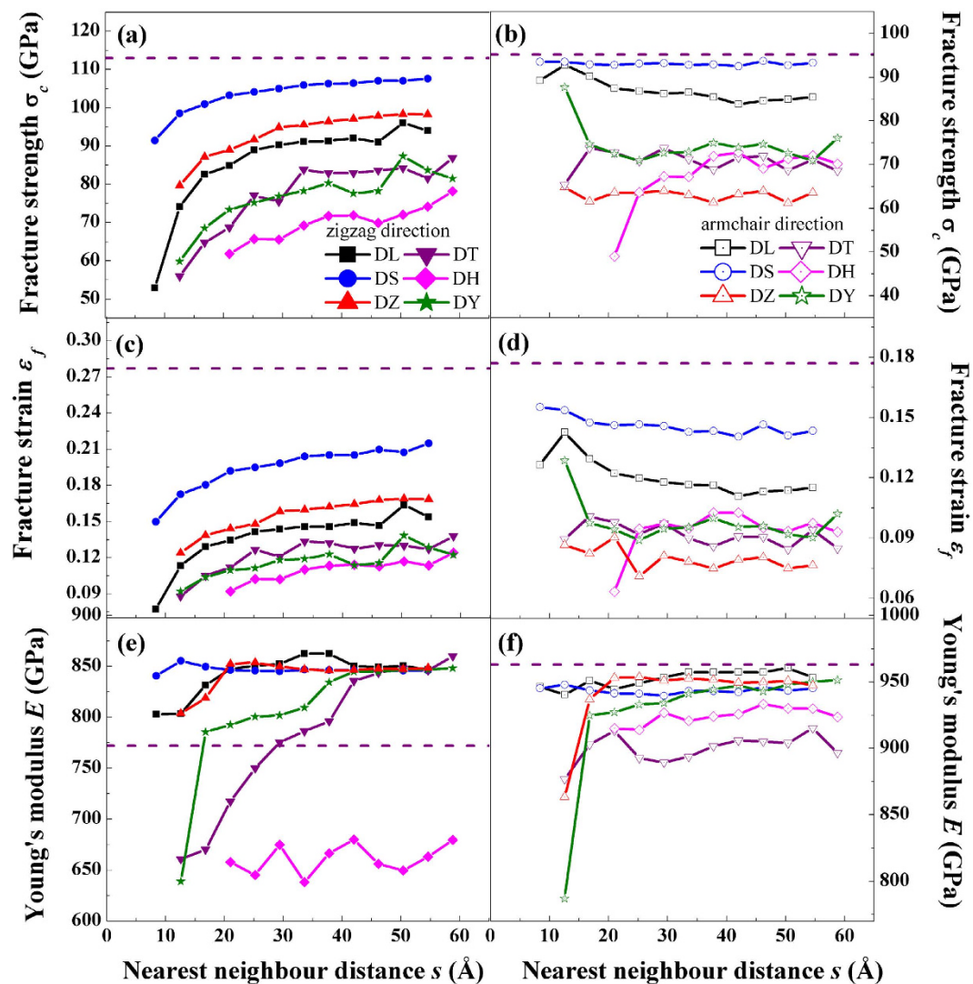
Figure 4. The mechanical properties of graphene with various defects. (a,b) The fracture strength ( \sigma_c ) versus the nearest neighbour distance ( s ); (c,d) The fracture strain ( \varepsilon_f ) versus s . (e,f) The Young's modulus ( E ) versus s . The solid (left) and open (right) symbols represent the loading direction in zigzag and armchair, respectively. The dash lines indicate the corresponding data of pristine graphene.
