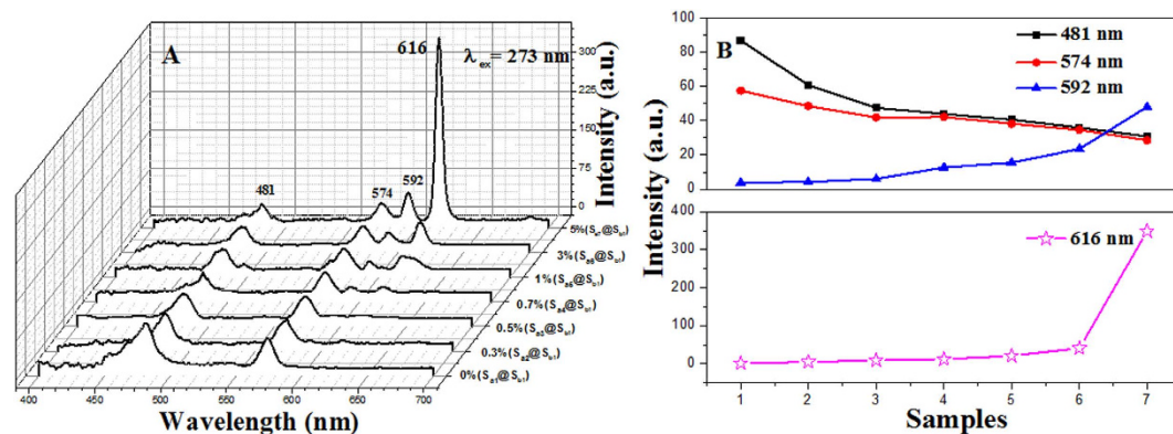
Figure 6. Emission spectra of samples S ax @S b1 (x=1-7) when the mass percentage of PANI is fixed as 30% and the mass ratio of Fe 3 O 4 to PMMA is fixed as 1:1 (A), dependence of the emission intensity on the various samples (B).
