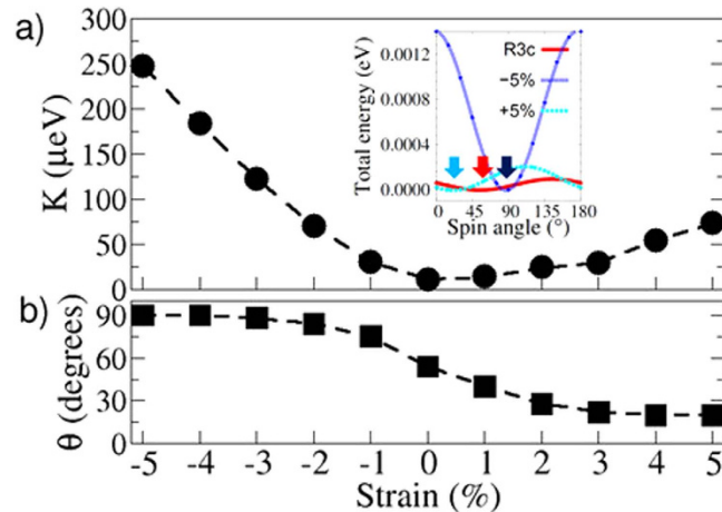
Figure 5. Calculated single ion anisotropy vector ( Kn ) as a function of applied epitaxial strain. (a) The magnitude and (b) The direction of the easy spin axis with respect to the z -axis. The inset shows the relative sinusoidal variations of the single ion anisotropy. The energy minimum (indicated with red arrow) for the bulk ground state corresponds to 54^\circ i.e. along the [111] direction. The applied epitaxial strain shifts the energy minimum (indicated using black and cyan arrows) toward the z -axis and the x - y plane for compressive and tensile strains, respectively.
