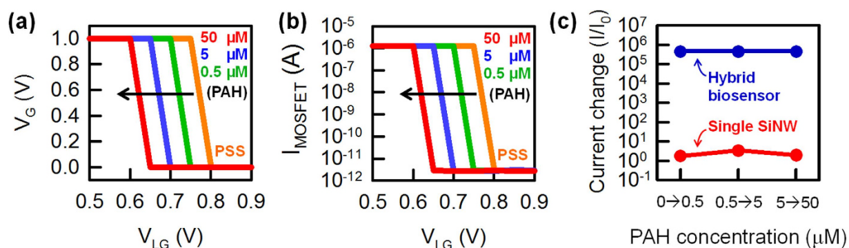
Figure 5. Measured electrical characteristics of the hybrid biosensor as a function of PAH concentration. (a) V_G - V_{\text{LG}} and (b) I_{\text{MOSFET}} - V_{\text{LG}} characteristics of the hybrid biosensor with varying PAH concentrations. (c) Comparison of the current change for the two biosensor types at different PAH concentrations.
