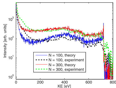
Figure 4. Volume integrated theoretical electron spectrum of x-ray irradiated Xe clusters of the average size of 100 and 300 atoms and the corresponding experimental results within the measured energy range. The photon energy is 5.5 keV and the peak fluence is 45 \mu\text{J}/\mu\text{m}^2 .
