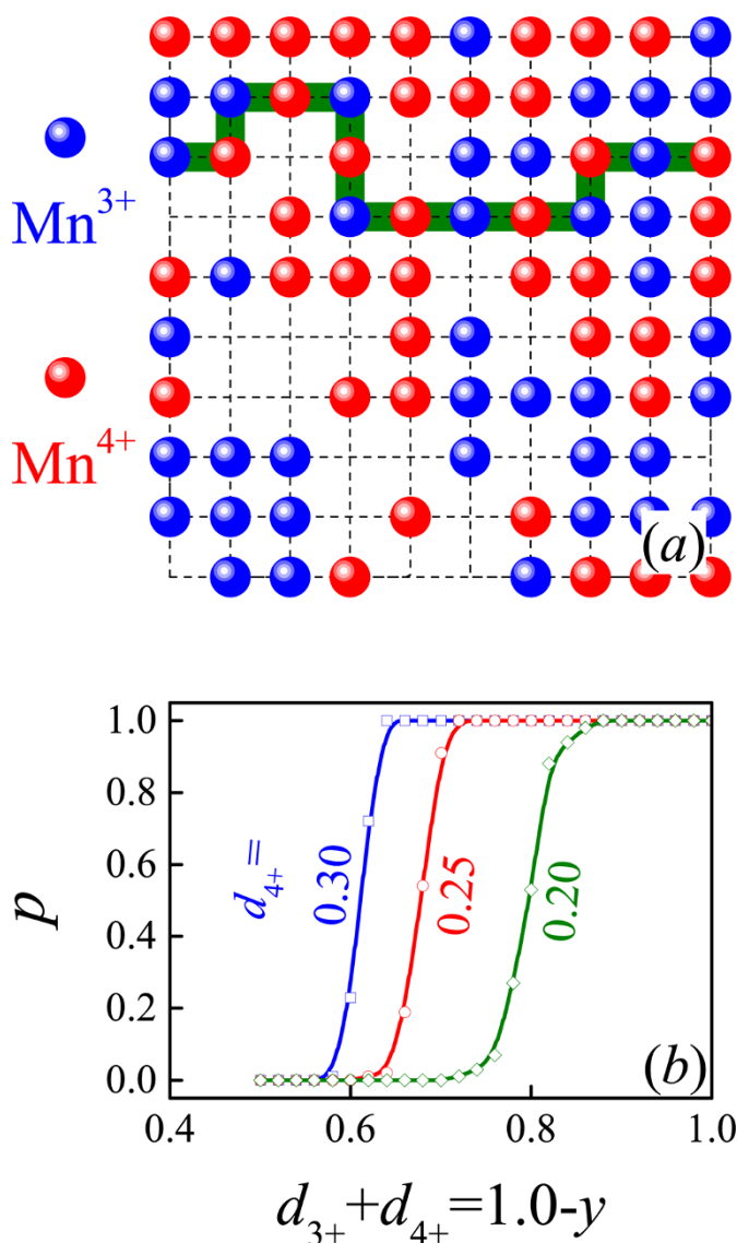
Figure 6 | (a) A two-dimensional section of a cubic lattice with random occupation of Mn^{3+} and Mn^{4+} , given fixed d_{3+} and d_{4+} . The olive pipe-like channel is conductive due to the alternating Mn^{3+} - Mn^{4+} occupation. (b) Simulated conduction probability p as a function of (d_{3+}+d_{4+}) given three different d_{4+} values as indicated. The abrupt change of p from 0.0 to 1.0 implies the conduction percolation.
