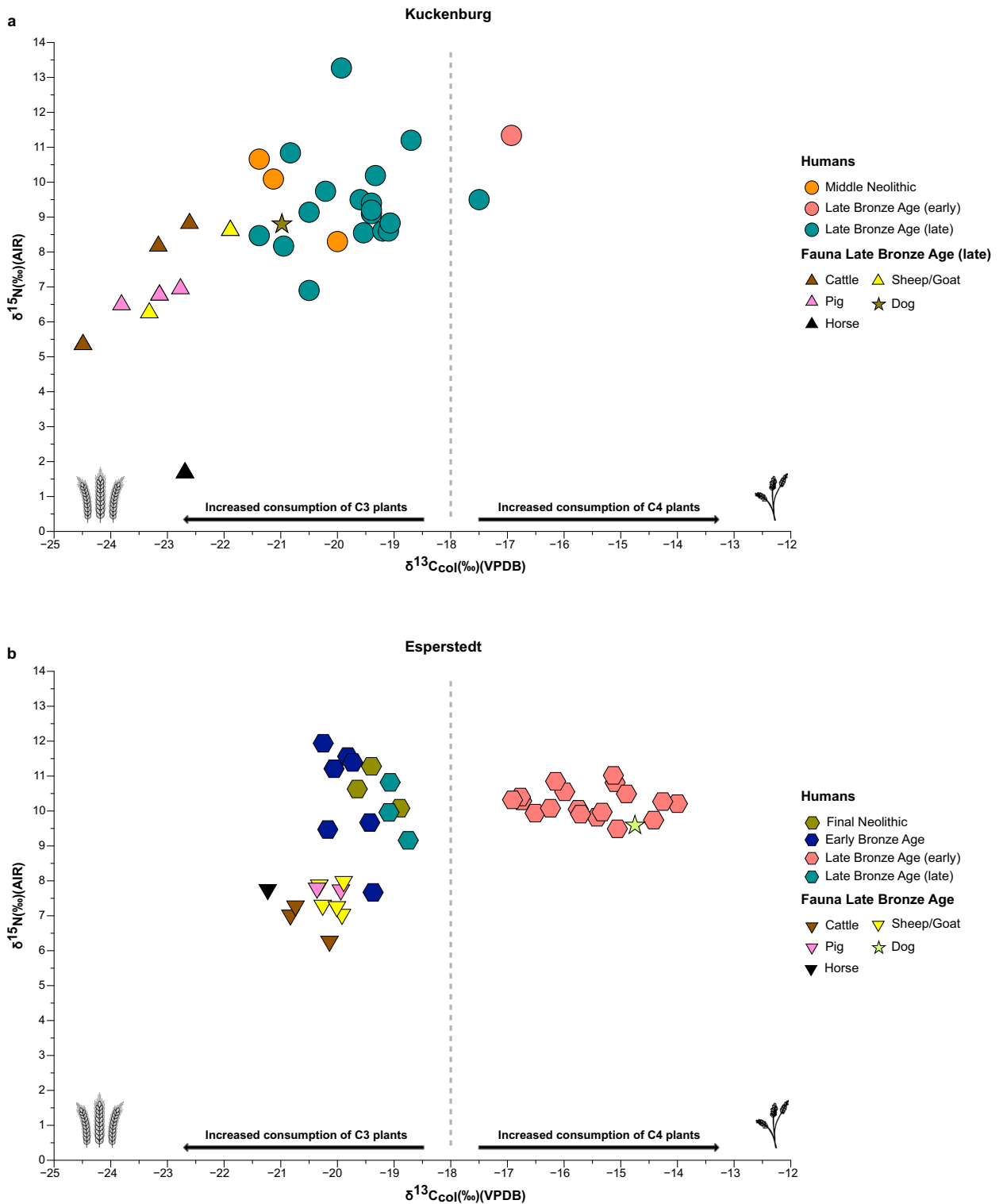
Figure 2. Comparison of \delta^{13}\text{C} and \delta^{15}\text{N} values from bone collagen for ancient individuals and fauna from Kuckenburg and Esperstedt. The dashed line represents millet's "threshold" of \delta^{13}\text{C} = -18\text{‰} 14,47 . (a) \delta^{13}\text{C} and \delta^{15}\text{N} values for Kuckenburg individuals and fauna. (b) \delta^{13}\text{C} and \delta^{15}\text{N} values for Esperstedt individuals and fauna. Wheat icon (left) was created by Oleksandr Panasovskiy from Noun Project (CC BY 3.0), https://thenounproject.com/browse/icons/term/wheat/ . Millet icon (right) was created by Roman from Noun Project (CC BY 3.0), https://thenounproject.com/browse/icons/term/millet/ .
