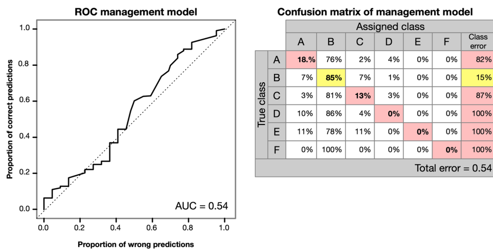
Figure 7. ROC curve of averaged random forest classifiers for the presence of Jacobaea aquatica in Bavaria with management parameters as predictors; and confusion matrix of the random forest classifiers for the frequency of the species in dependency of management factors.
