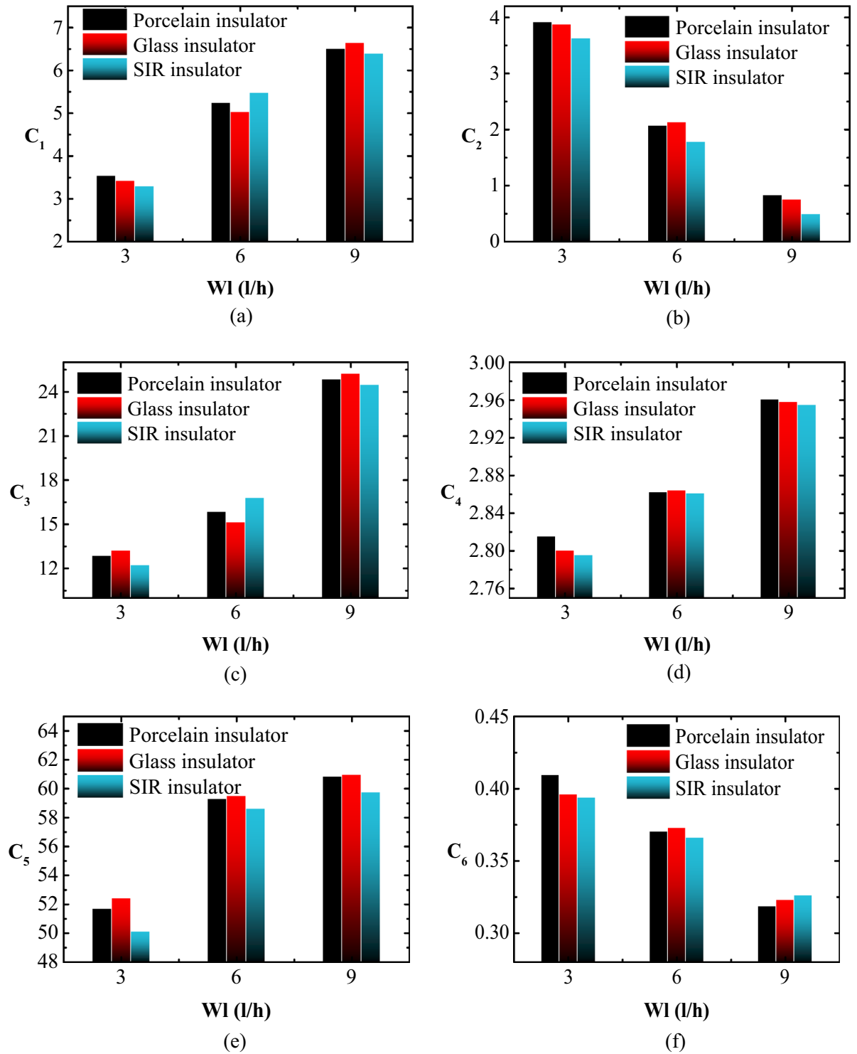
Figure 12. LC indicators versus Wt for tested insulators under SDD=0.2 mg/cm 2 , NSDD=0.35 mg/cm 2 and P u /P L =1/1: (a) C 1 ; (b) C 2 ; (c) C 3 ; (d) C 4 ; (e) C 5 ; (f) C 6 .
