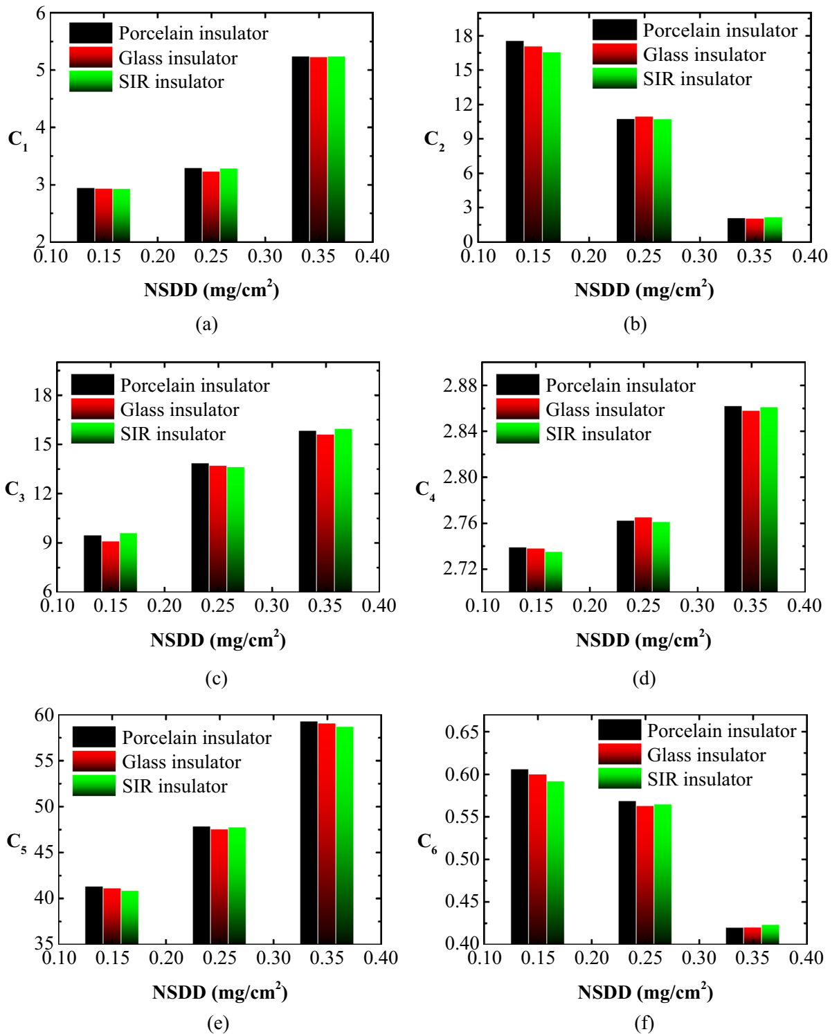
Figure 11. LC indicators versus NSDD for tested insulators under SDD=0.2 mg/cm 2 , Wt=9 l/h and P u /P L =1/1: (a) C 1 ; (b) C 2 ; (c) C 3 ; (d) C 4 ; (e) C 5 ; (f) C 6 .
