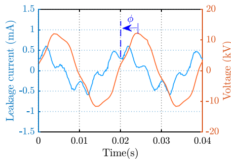
Figure 5. The phase difference between leakage current and applied voltage.
