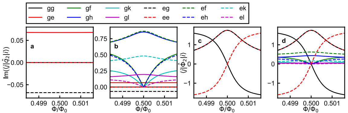
Figure 6. Numerically calculated matrix elements \langle j|\hat{q}_2|i\rangle for i = g, e and (a) j = g, e , (b) j = g, e, f, h, k, l , where |f\rangle, |h\rangle, |k\rangle, and |l\rangle respectively represent the second, third, fourth, and fifth excited states of \hat{\mathcal{H}}_2 . Numerically calculated matrix elements \langle j|\hat{\Phi}_2|i\rangle for i = g, e and (c) j = g, e , (d) j = g, e, f, h, k, l . Note that the x axis ranges are smaller than those in Fig. 4.
