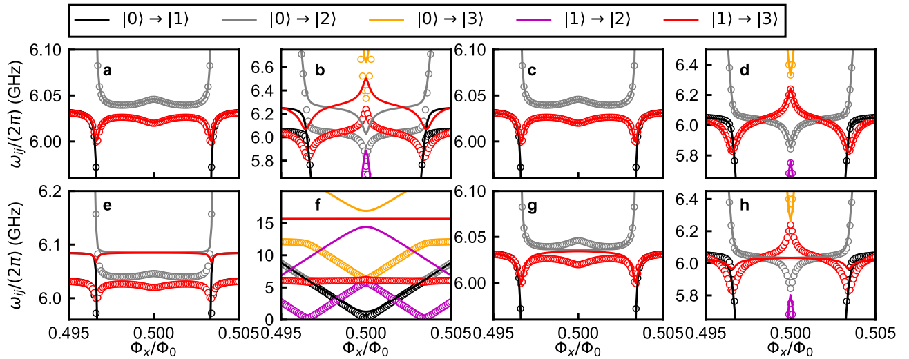
Figure 4. Transition frequencies of the qubit-oscillator circuit fitted with different approximate Hamiltonians. Numerically calculated transition frequencies from \hat{\mathcal{H}}_{circ} are plotted as circles while the fitting spectra are plotted as lines. Two mutual inductance values, corresponding to different qubit-oscillator coupling strengths, are used: L_c = 20 pH (a,c,e,g) and L_c = 350 pH (b,d,f,h). The spectra are fitted with \hat{\mathcal{H}}_R (a–d) and \hat{\mathcal{H}}'_R (e–h). (a,b) The parameters of \hat{\mathcal{H}}_R are obtained from the relations described in Table 1: \omega/(2\pi) = 6.033 GHz, \Delta_q/(2\pi) = 1.240 GHz, g/(2\pi) = 0.424 GHz, and I_p = 281.3 nA for L_c = 20 pH and \omega/(2\pi) = 6.272 GHz, \Delta_q/(2\pi) = 2.139 GHz, g/(2\pi) = 7.338 GHz, and I_p = 282.5 nA for L_c = 350 pH. (c,d) The parameters of \hat{\mathcal{H}}_R are obtained by fitting the spectra of \hat{\mathcal{H}}_{circ} to \hat{\mathcal{H}}_R : \omega/(2\pi) = 6.033 GHz, \Delta_q/(2\pi) = 1.240 GHz, g/(2\pi) = 0.430 GHz, and I_p = 281.3 nA for L_c = 20 pH and \omega/(2\pi) = 6.064 GHz, \Delta_q/(2\pi) = 2.388 GHz, g/(2\pi) = 7.822 GHz, and I_p = 282.9 nA for L_c = 350 pH. (e,f) The parameters of \hat{\mathcal{H}}'_R are obtained from the circuit parameters of \hat{\mathcal{H}}'_{circ} in the similar way as in Table 1: \omega/(2\pi) = 6.085 GHz, \Delta_q/(2\pi) = 1.238 GHz, g'/(2\pi) = 0.043 GHz, and I_p = 281.3 nA for L_c = 20 pH, and \omega/(2\pi) = 15.66 GHz, \Delta_q/(2\pi) = 1.238 GHz, g'/(2\pi) = 0.492 GHz, and I_p = 281.3 nA for L_c = 350 pH. (g,h) The parameters of \hat{\mathcal{H}}'_R are obtained by fitting the spectra of \hat{\mathcal{H}}_{circ} to \hat{\mathcal{H}}'_R : \omega/(2\pi) = 6.035 GHz, \Delta_q/(2\pi) = 1.220 GHz, g/(2\pi) = 0.089 GHz, and I_p = 281.3 nA for L_c = 20 pH and \omega/(2\pi) = 6.034 GHz, \Delta_q/(2\pi) = 0.233 GHz, g/(2\pi) = 0.165 GHz, and I_p = 281.4 nA for L_c = 350 pH. Black, gray, orange, magenta, and red colors indicate transitions |0\rangle \rightarrow |1\rangle , |0\rangle \rightarrow |2\rangle , |0\rangle \rightarrow |3\rangle , |1\rangle \rightarrow |2\rangle , and |1\rangle \rightarrow |3\rangle , respectively.
